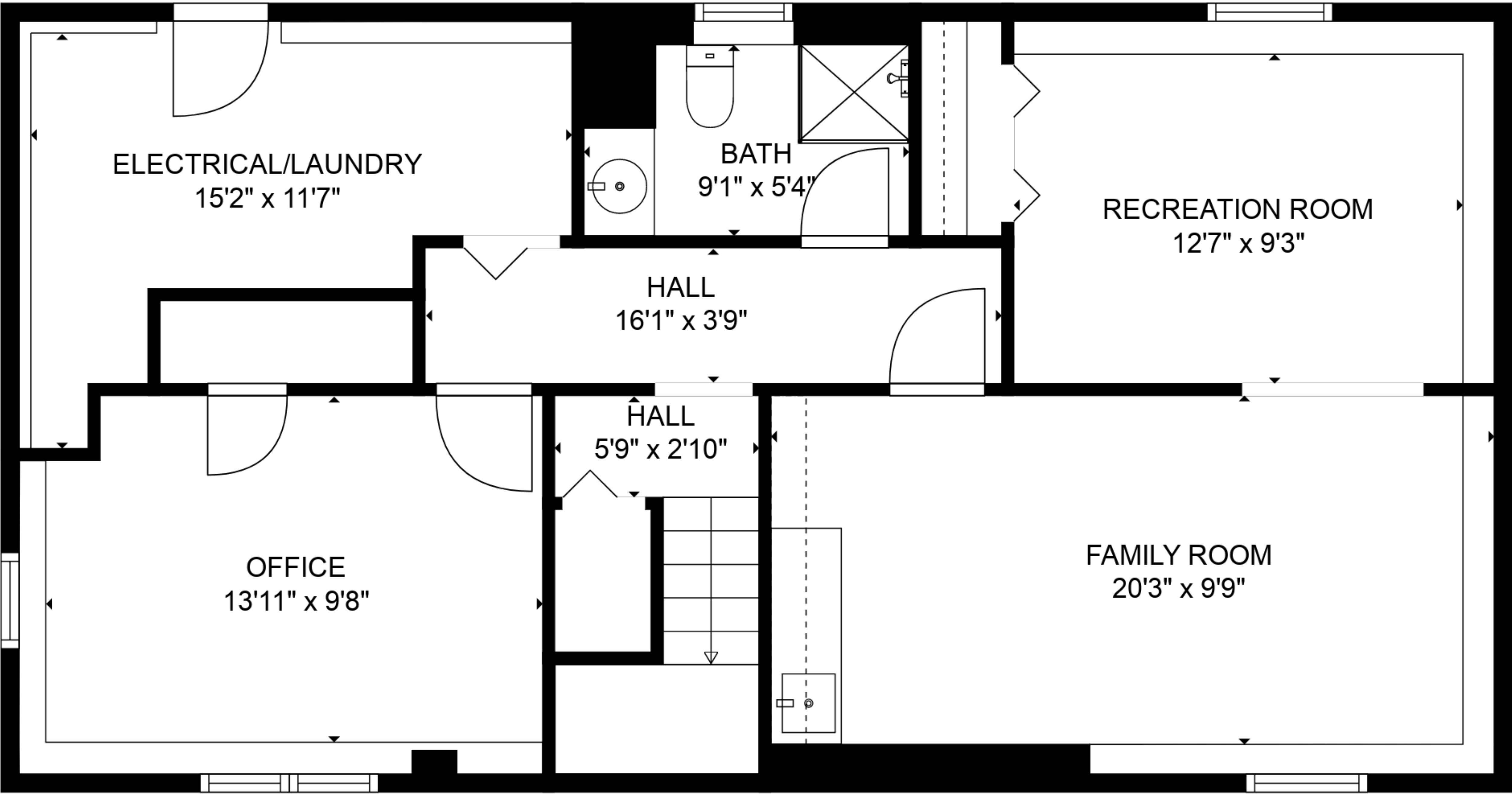
FLOOR 2
