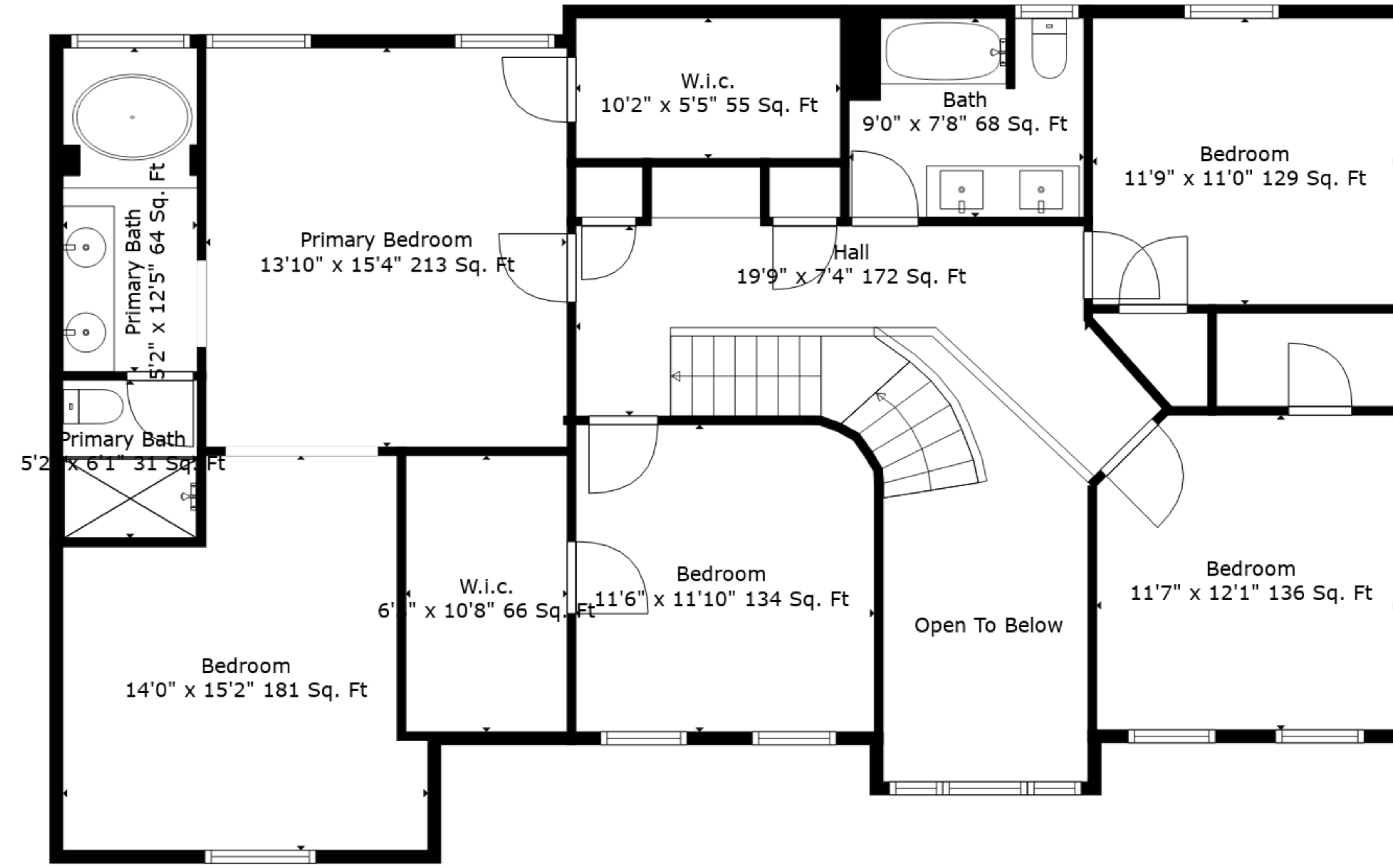
Floor 3
