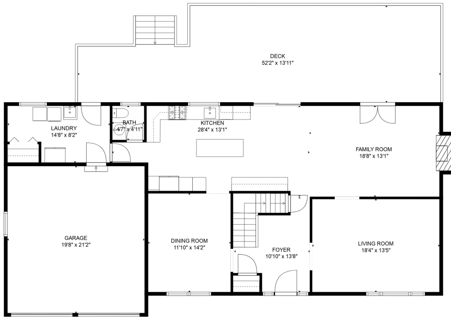
FLOOR 2
