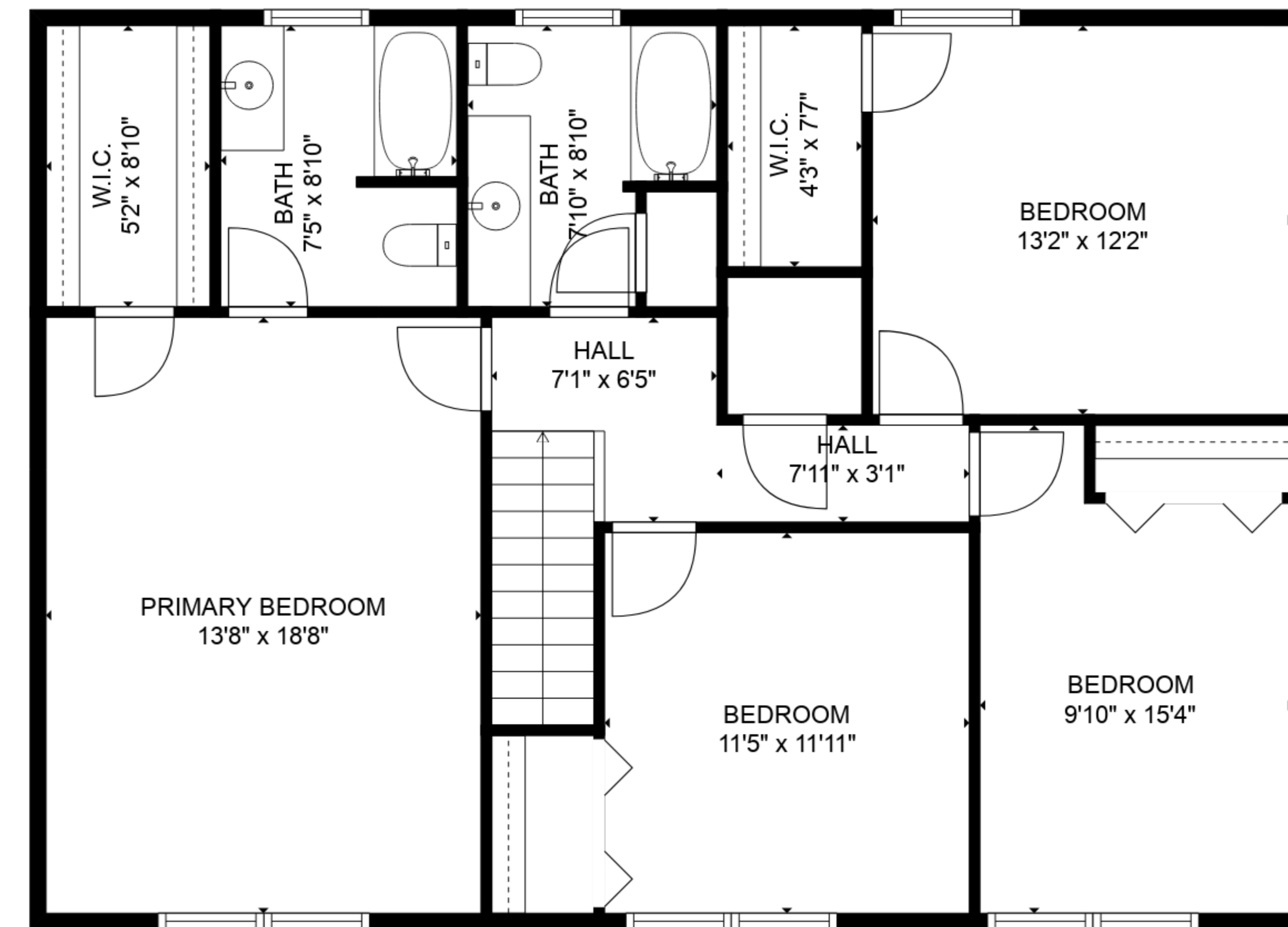
FLOOR 3
