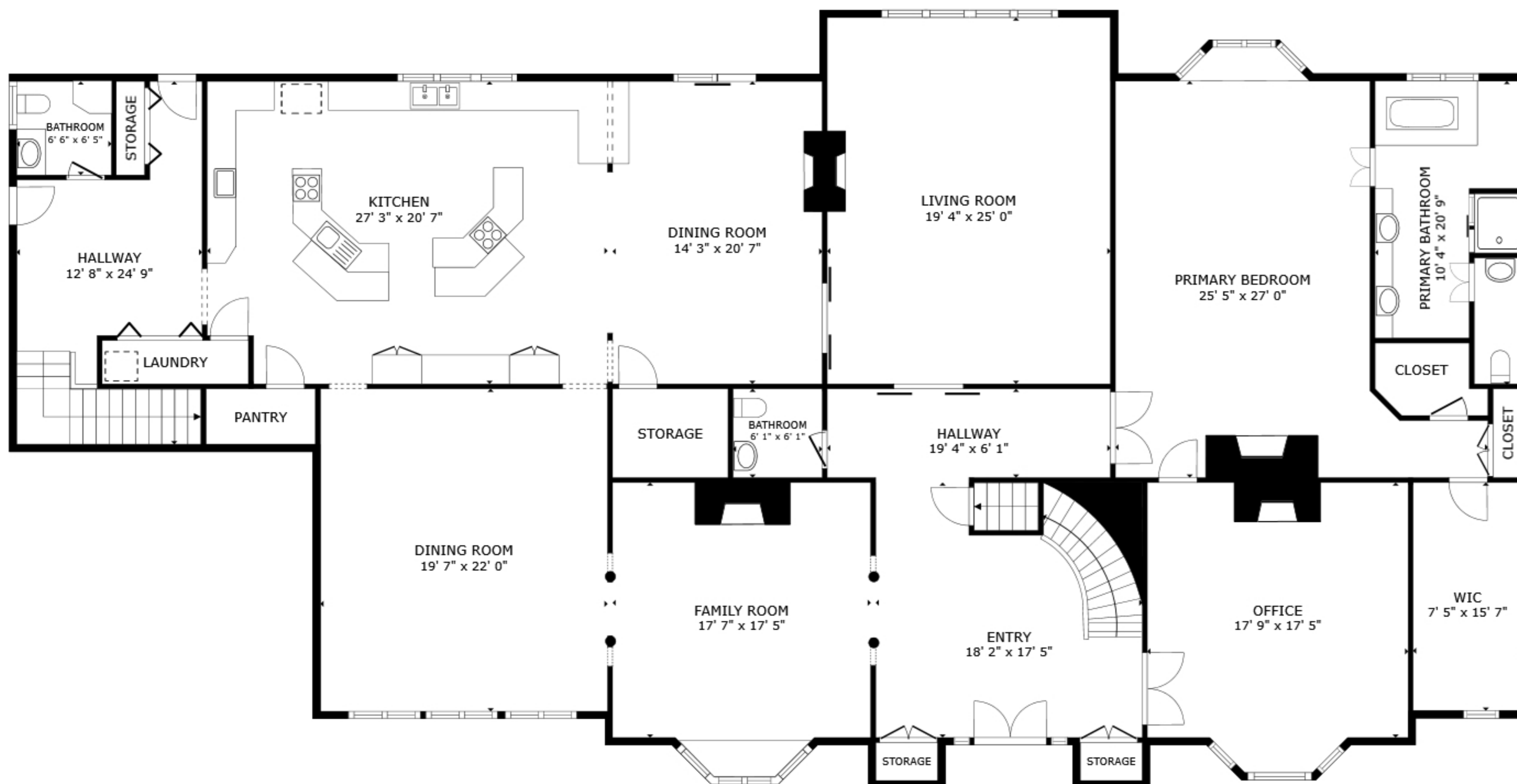
FLOOR 2
