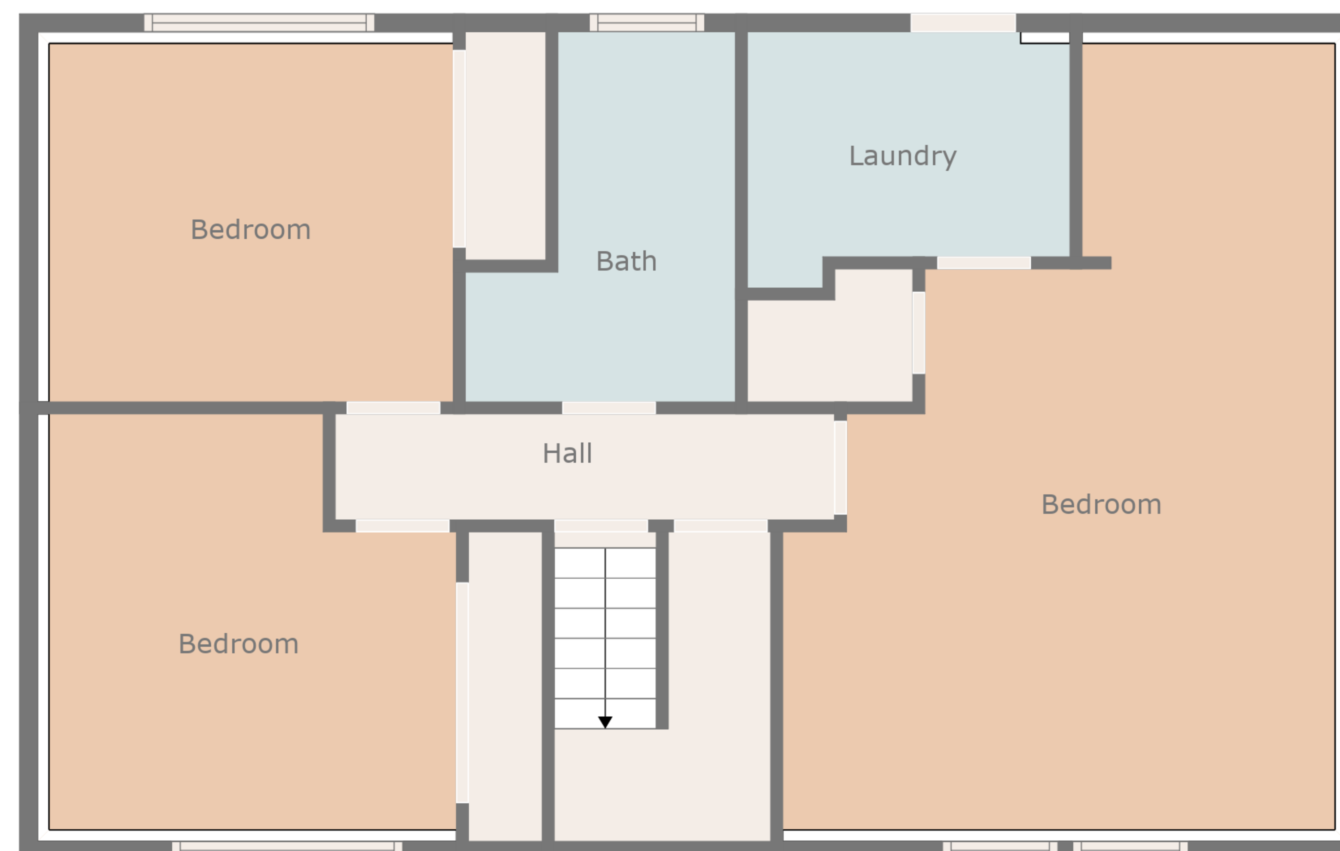
Floor 2
