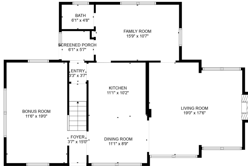
FLOOR 1
