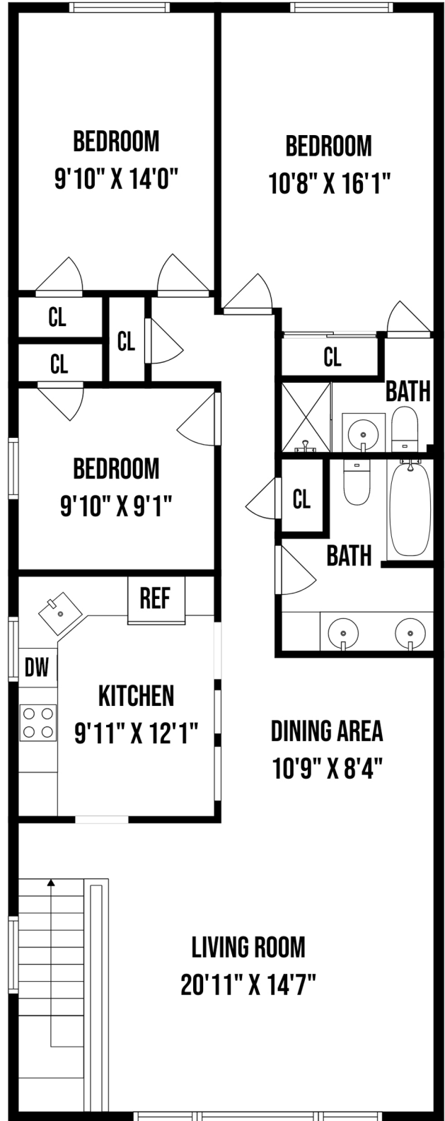
SECOND FLOOR
