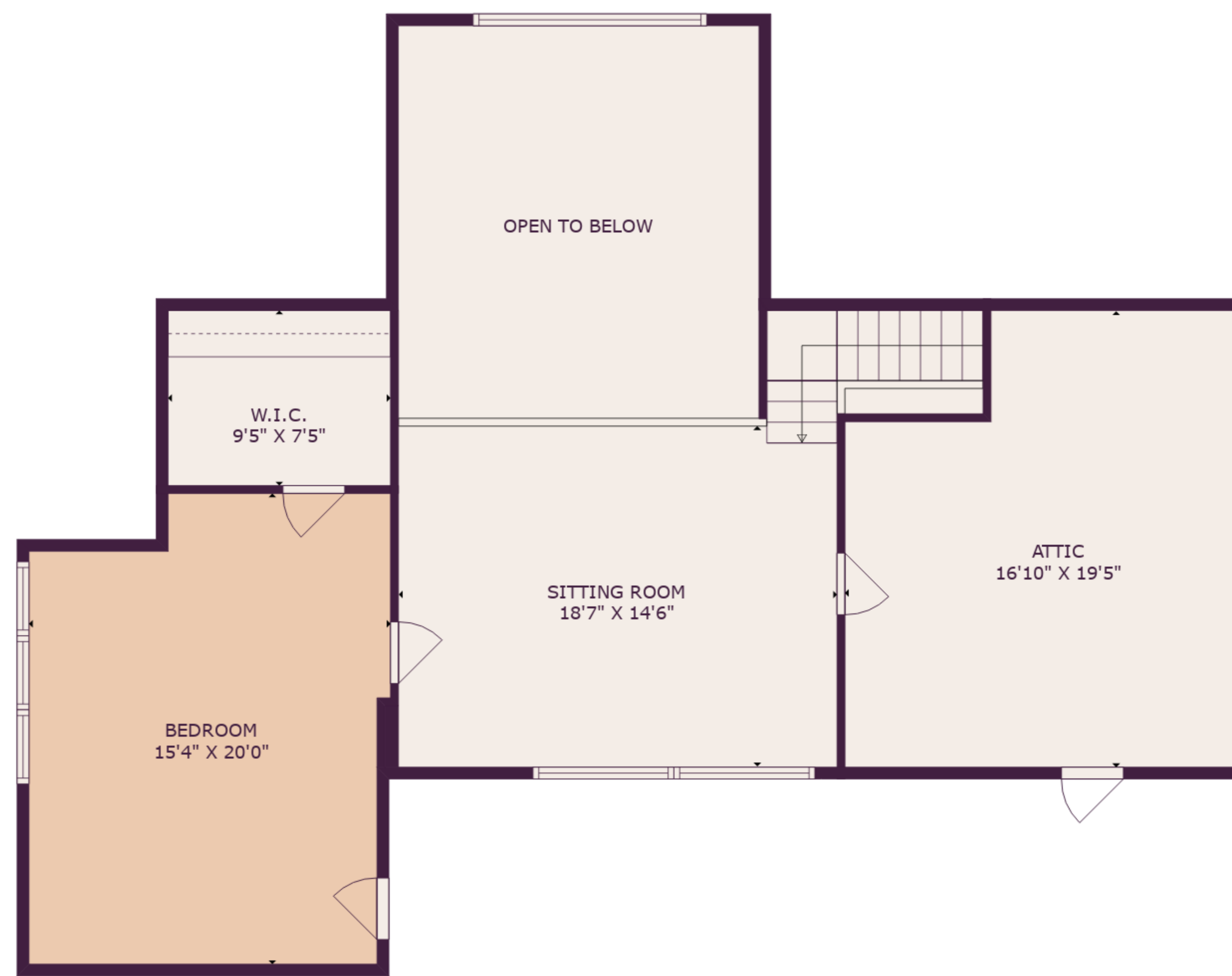
FLOOR 2
