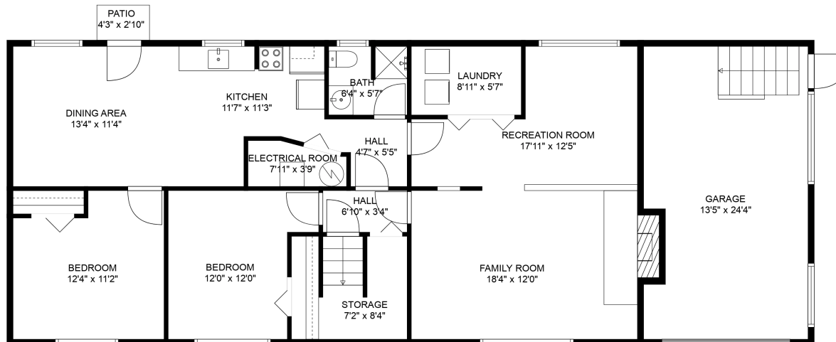
FLOOR 2
