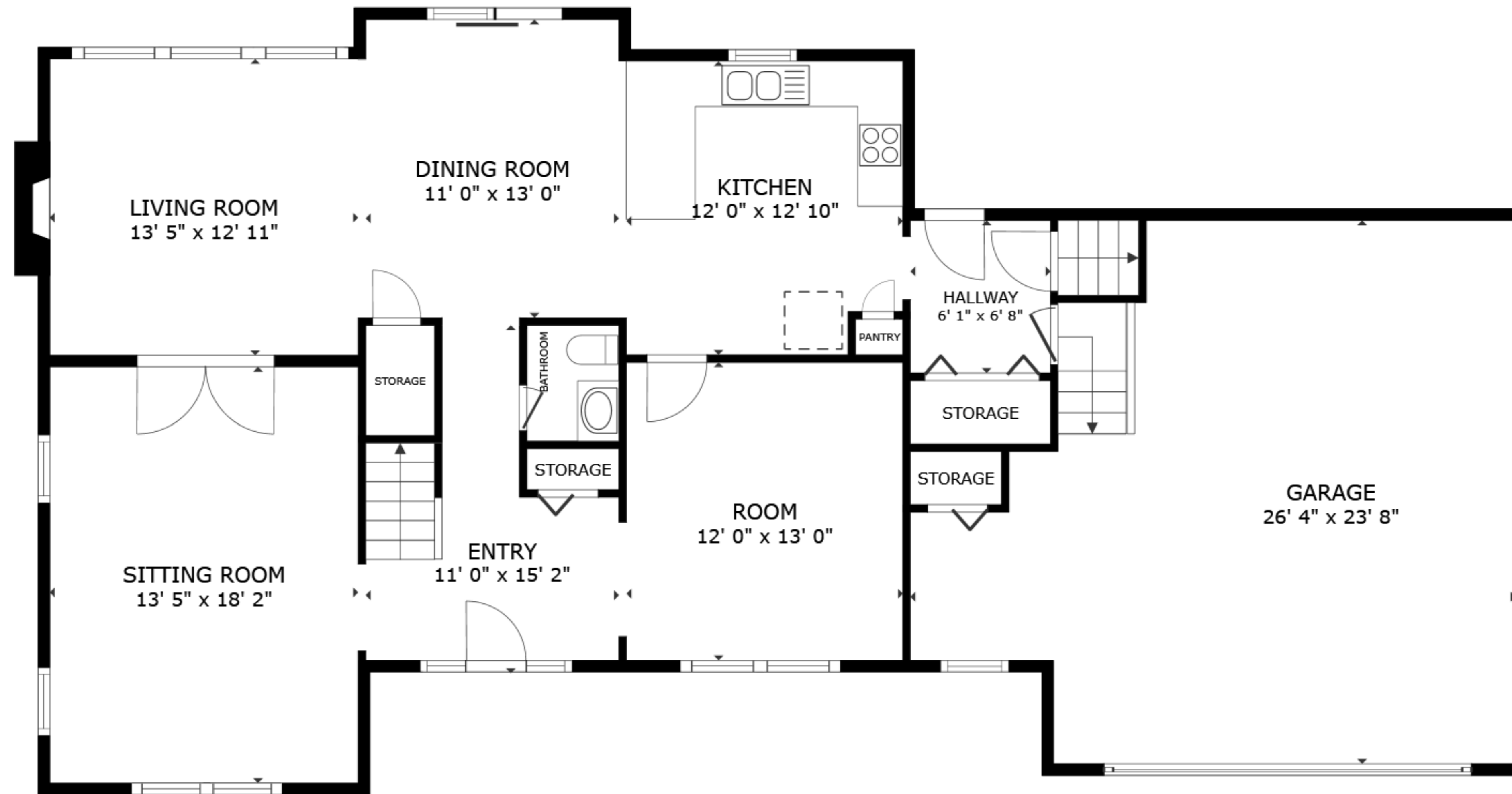
FLOOR 1
