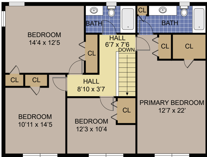
THIRD FLOOR
