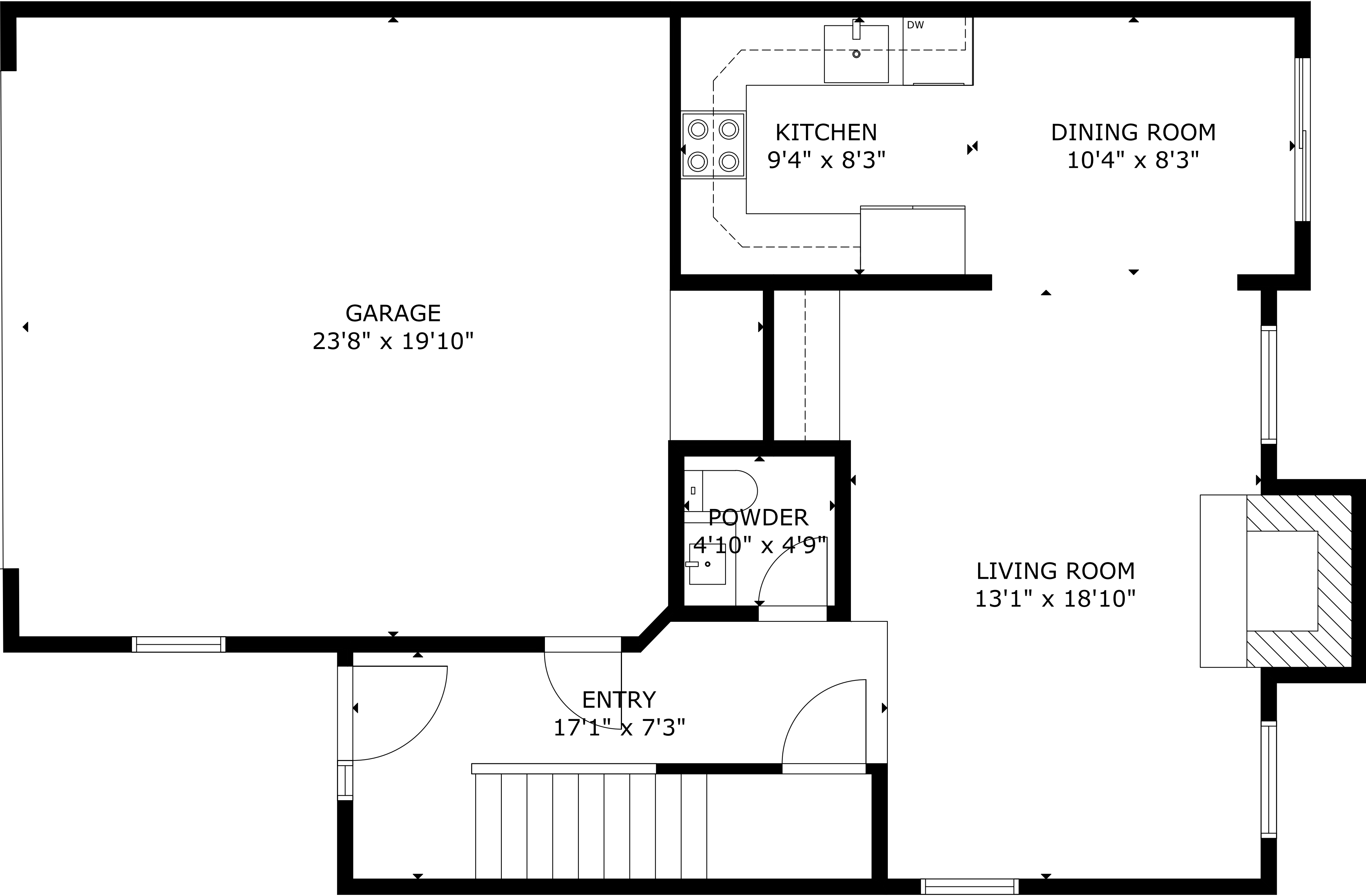
FLOOR 1
