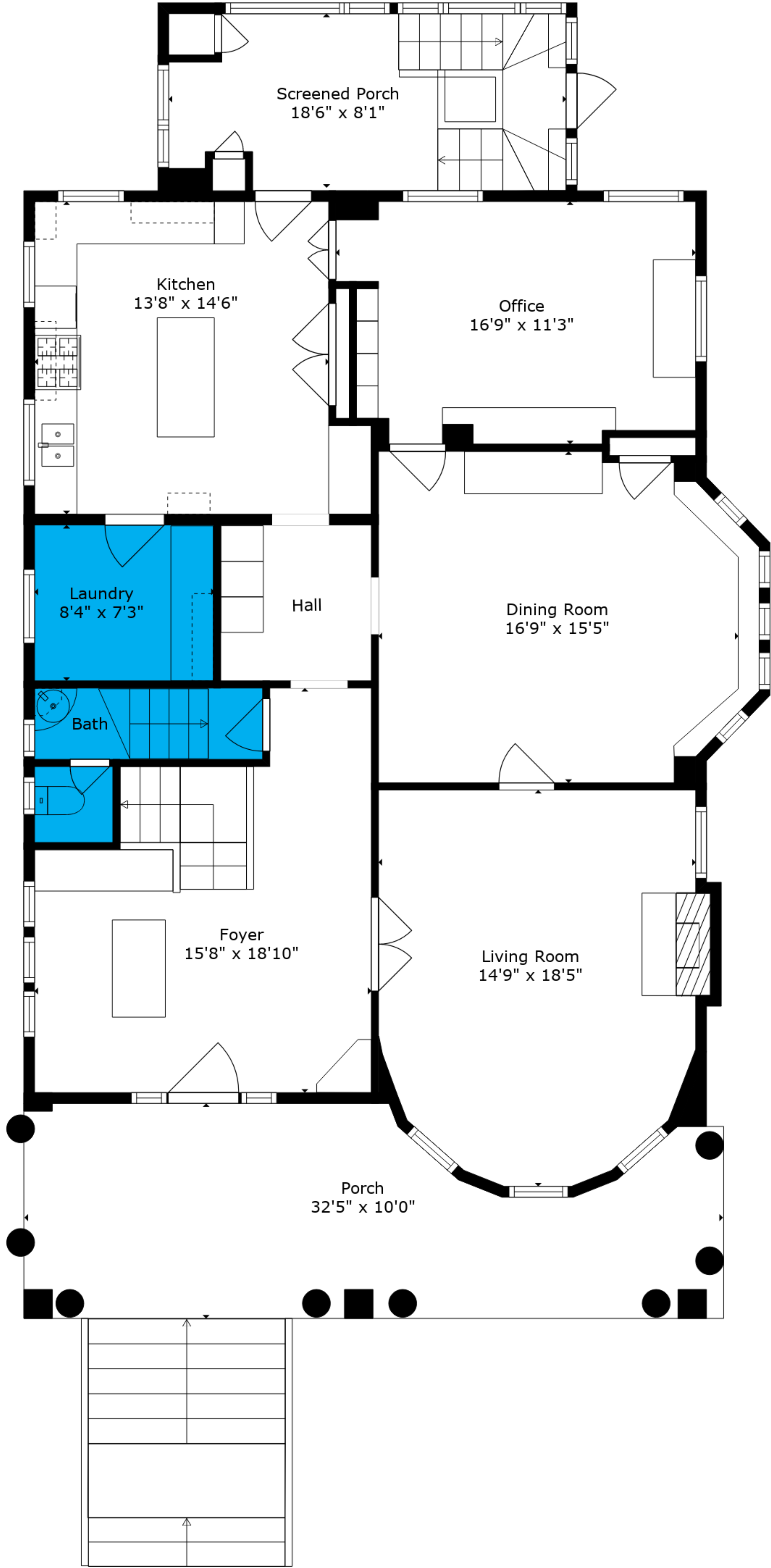
Floor 2
