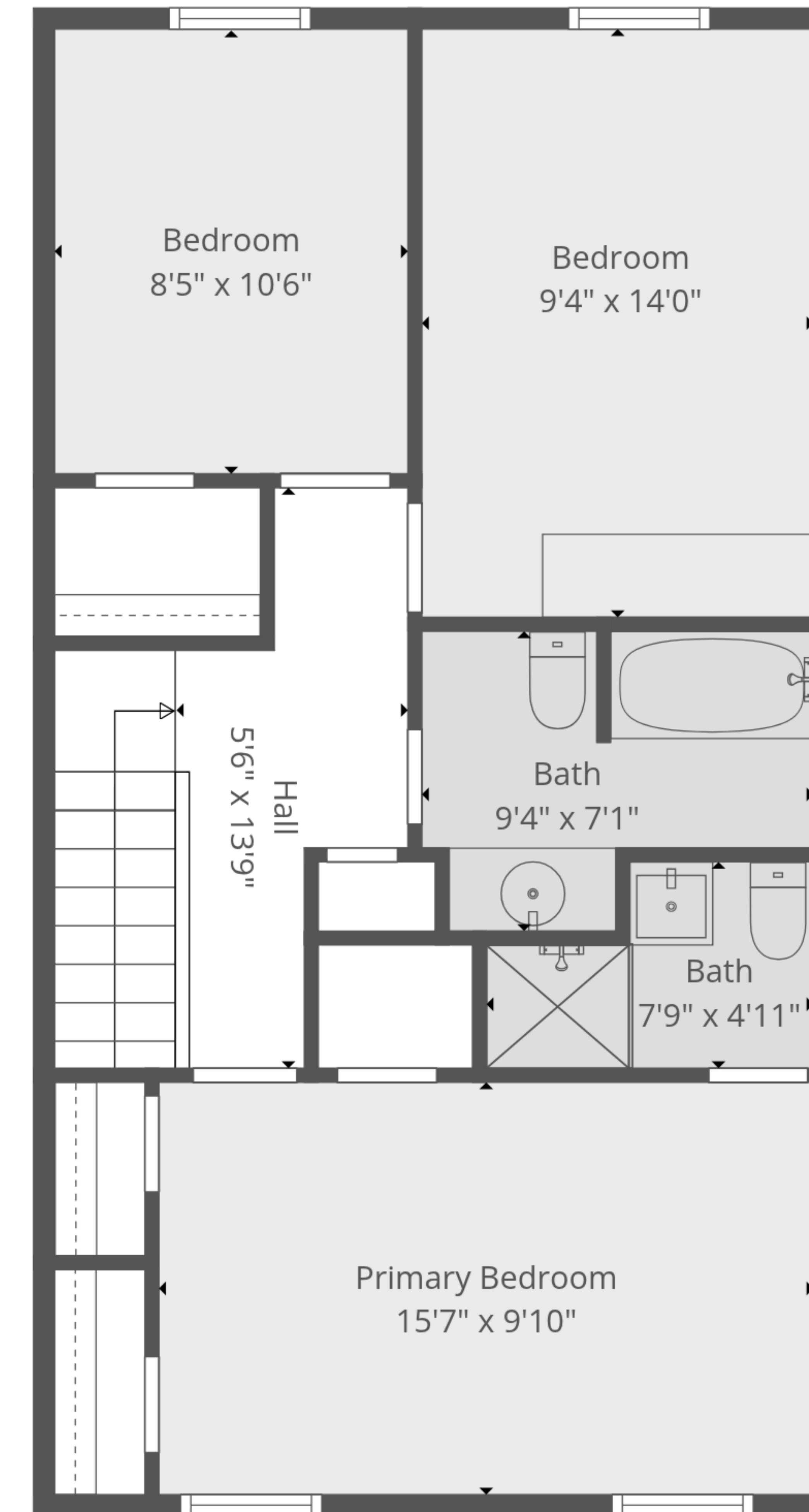
3rd Floor
