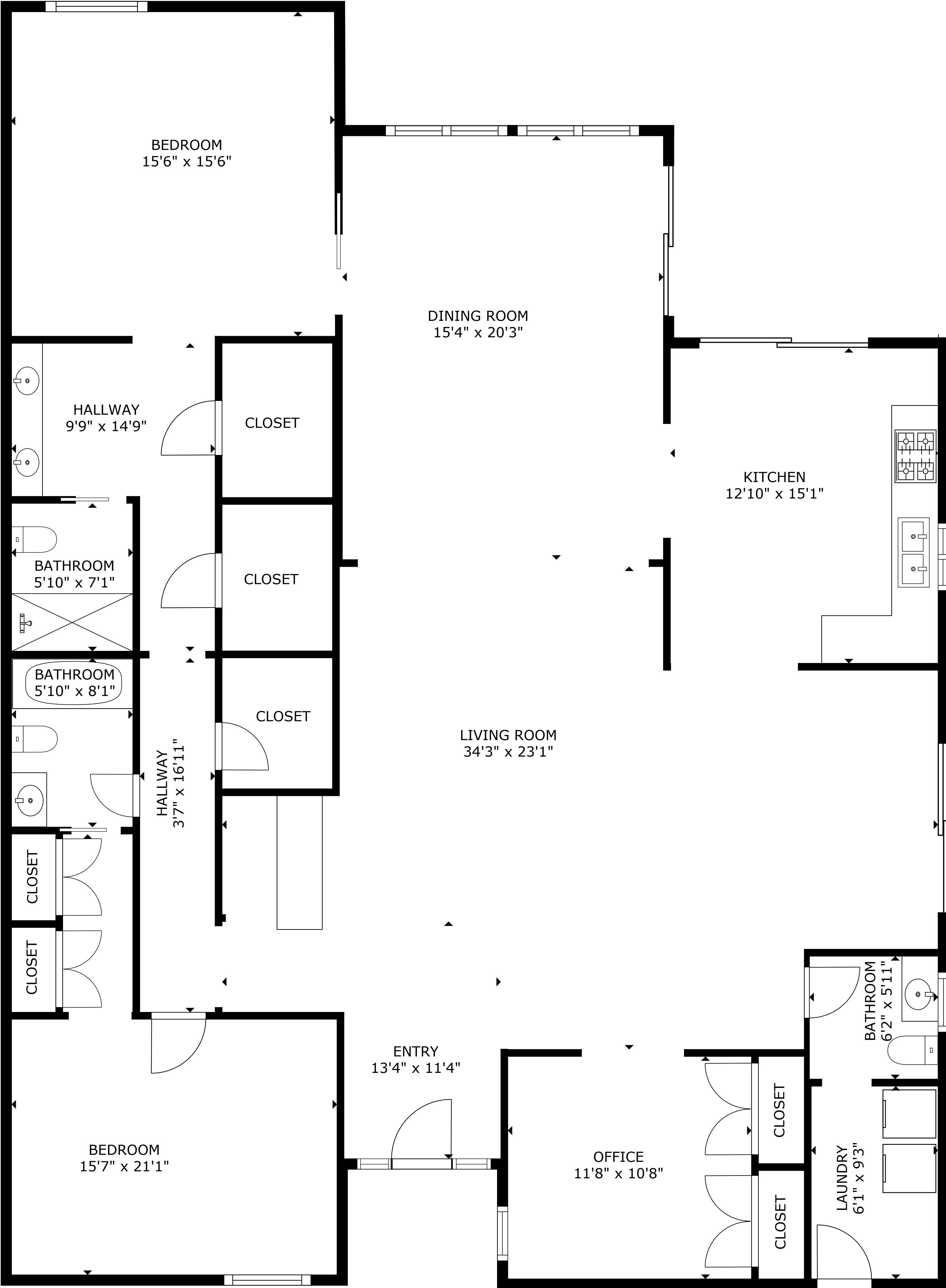
FLOOR PLAN
