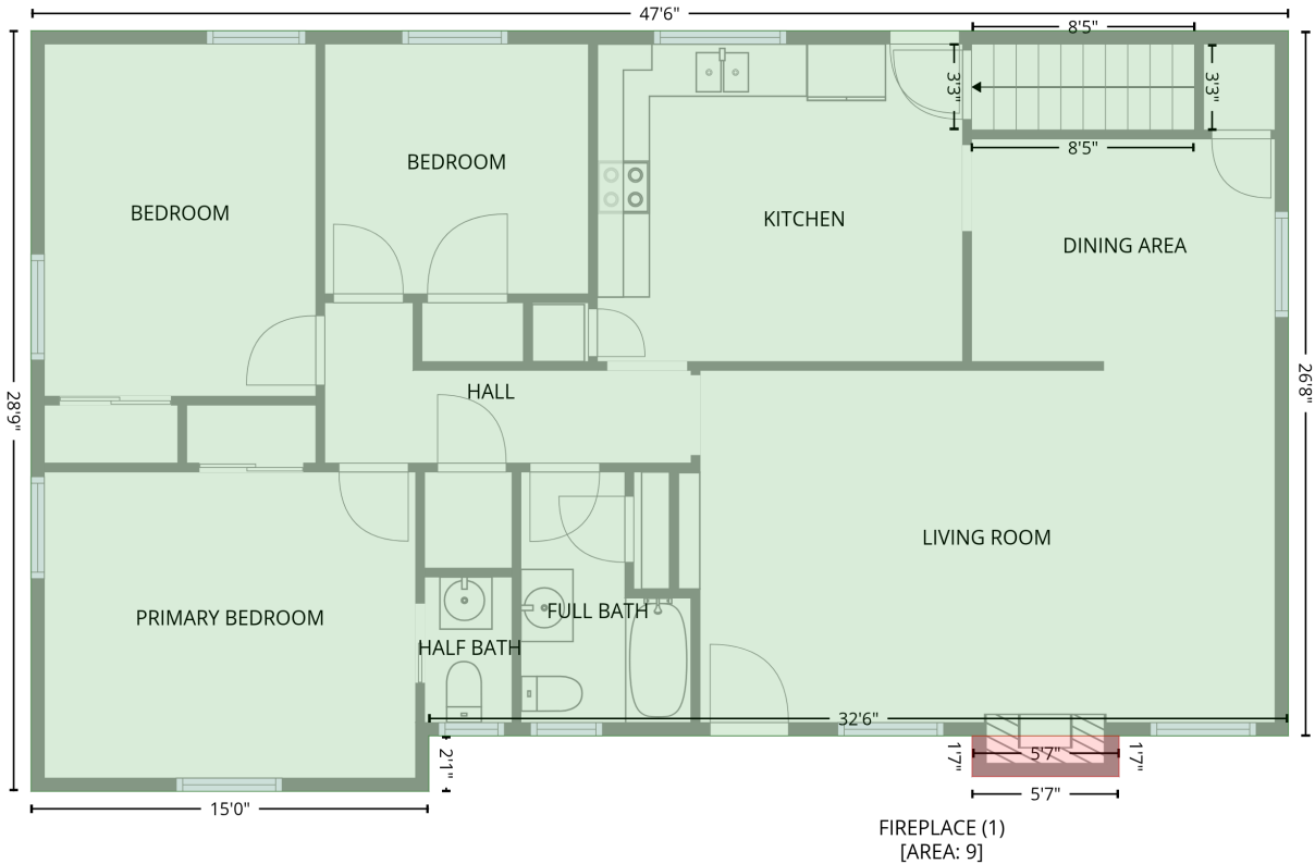
FLOOR 2 [AREA: 1298]
