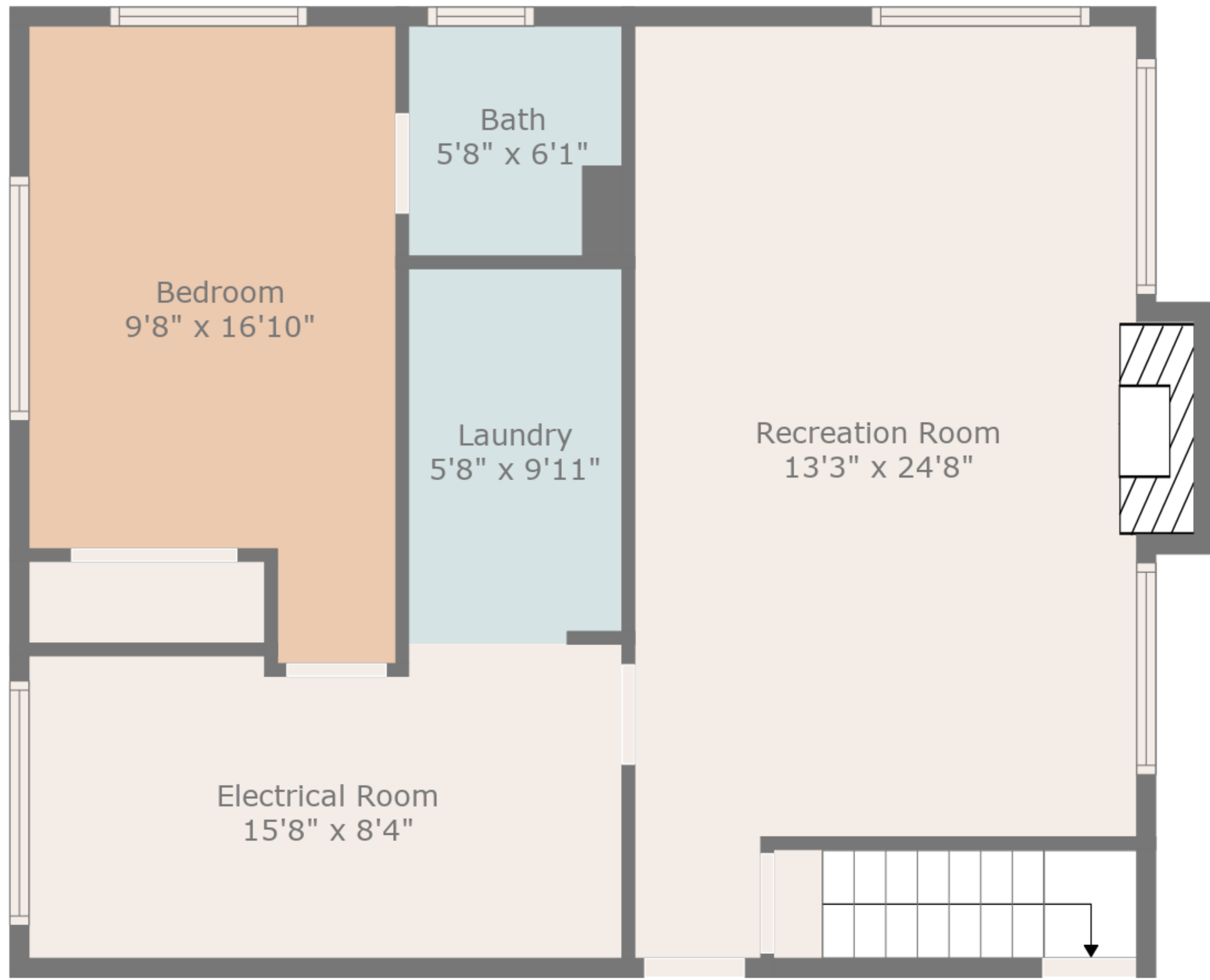
Floor 1
