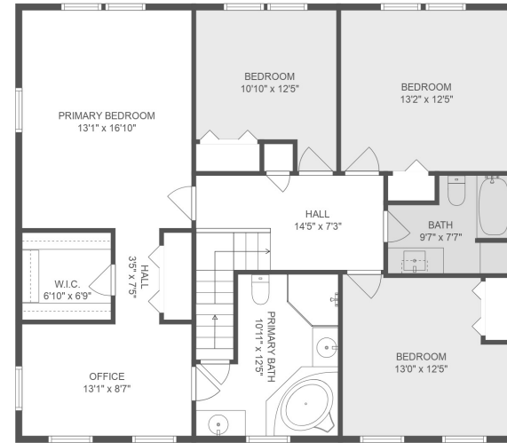
FLOOR 3
