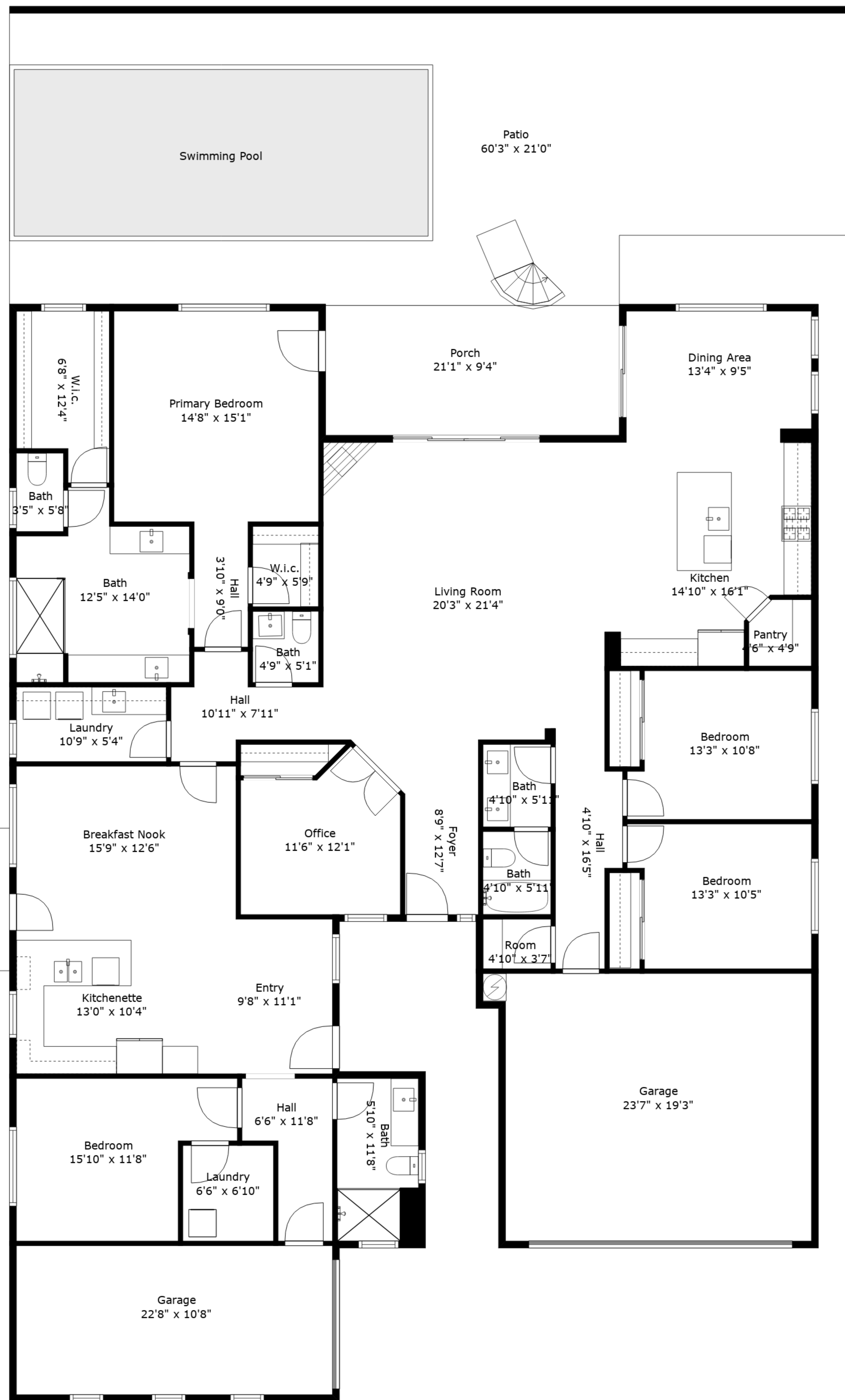
Floor 1
