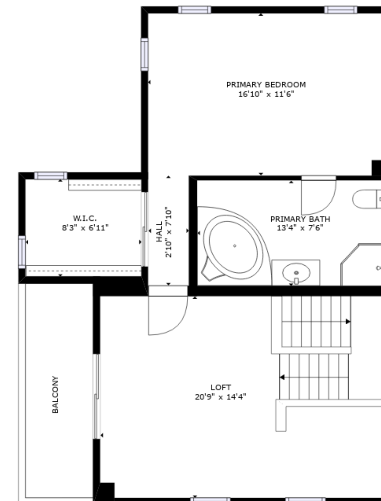
FLOOR 2
