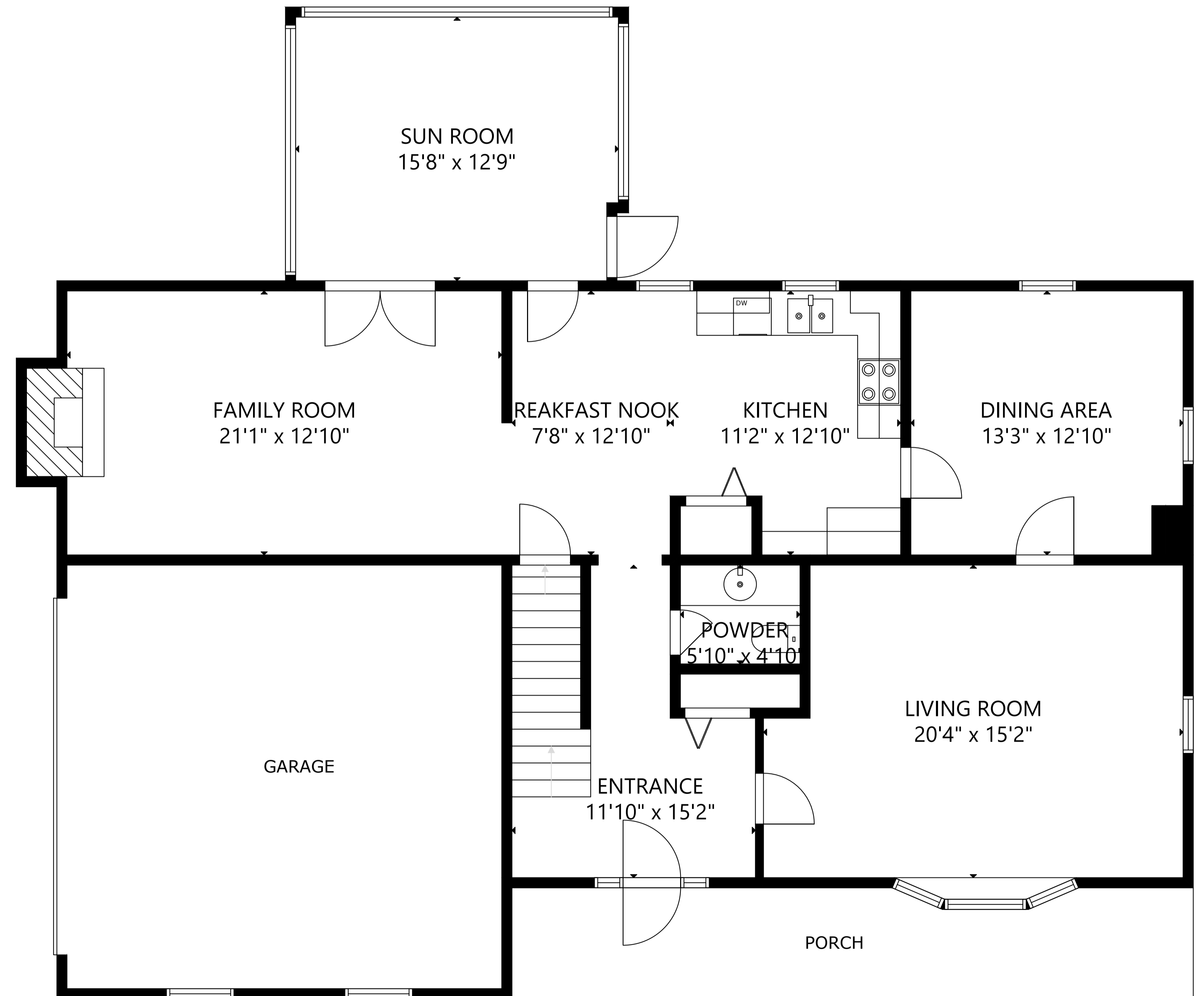
MAIN FLOOR
