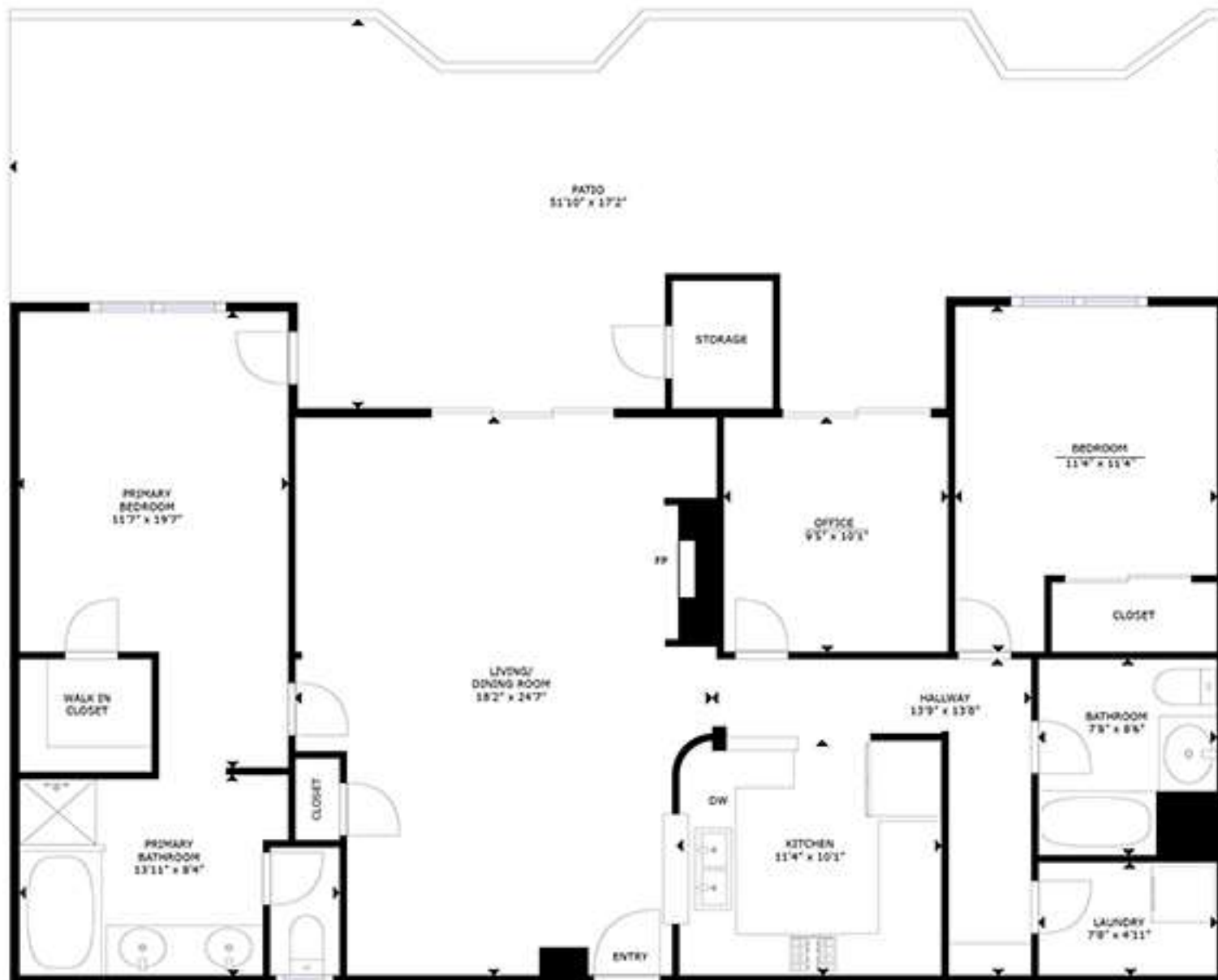
FLOOR PLAN
