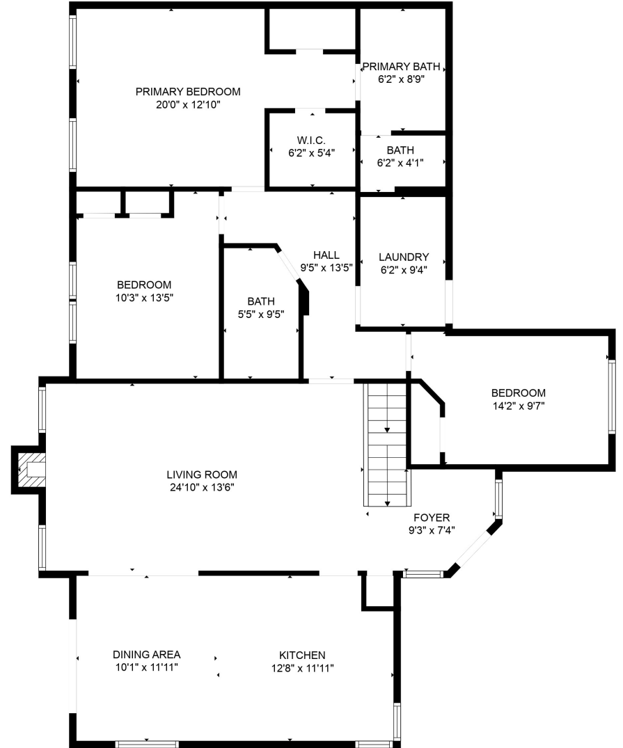
FLOOR 2
