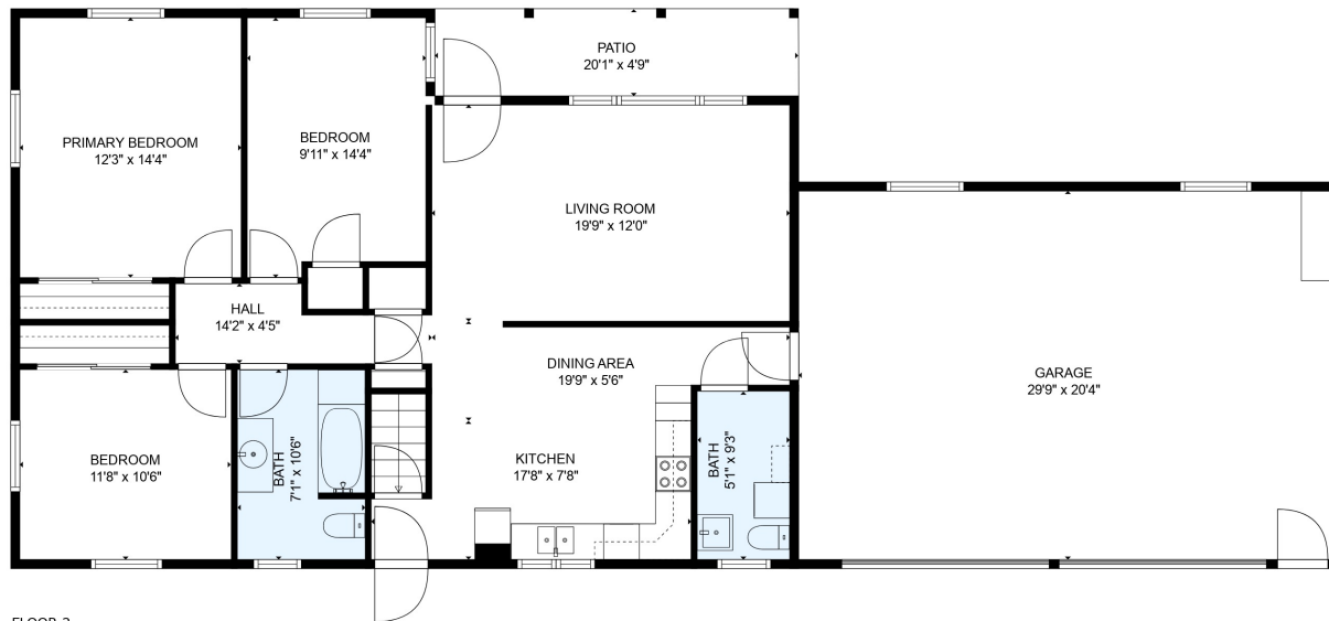
FLOOR 2
