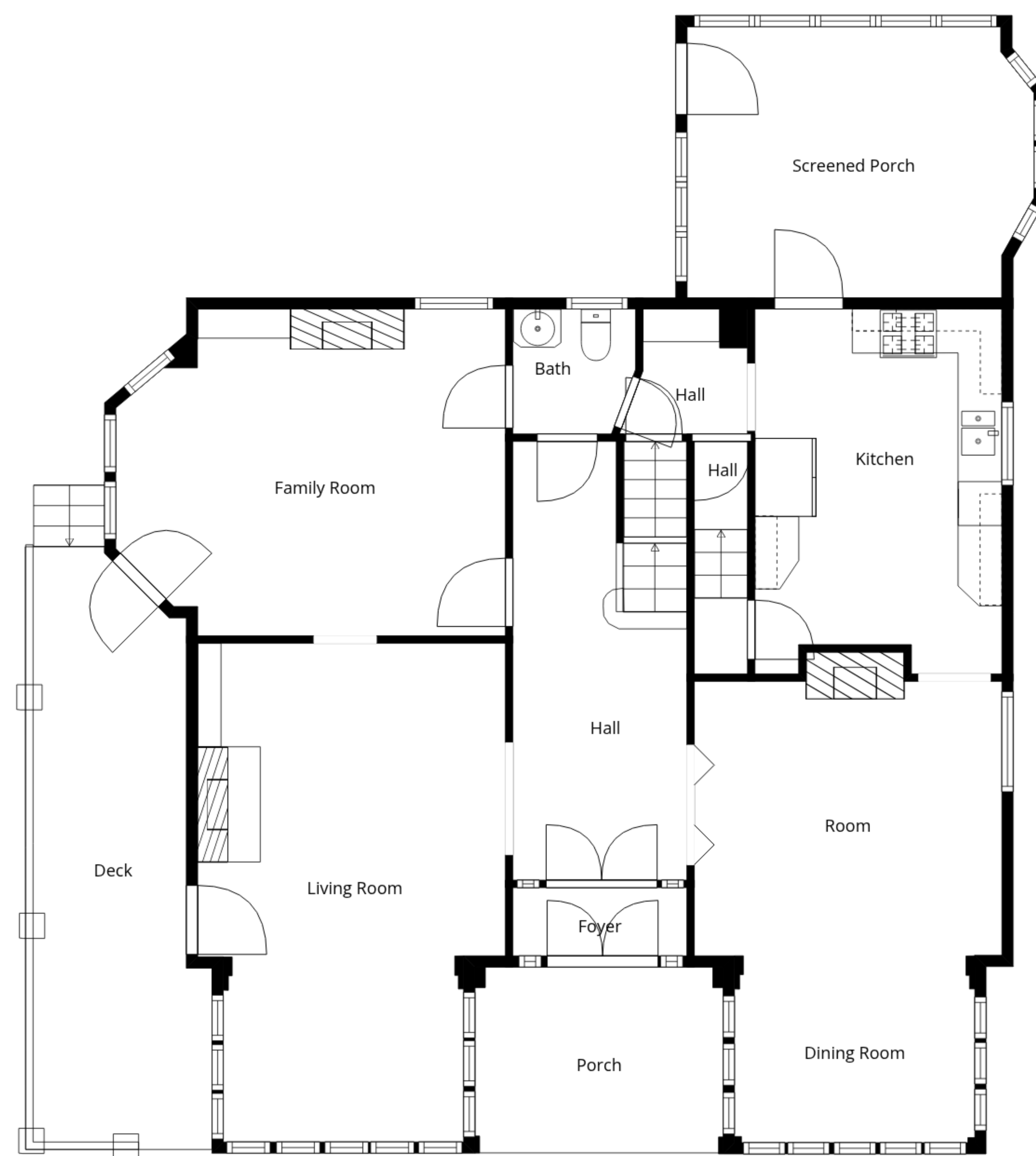
Floor 2
