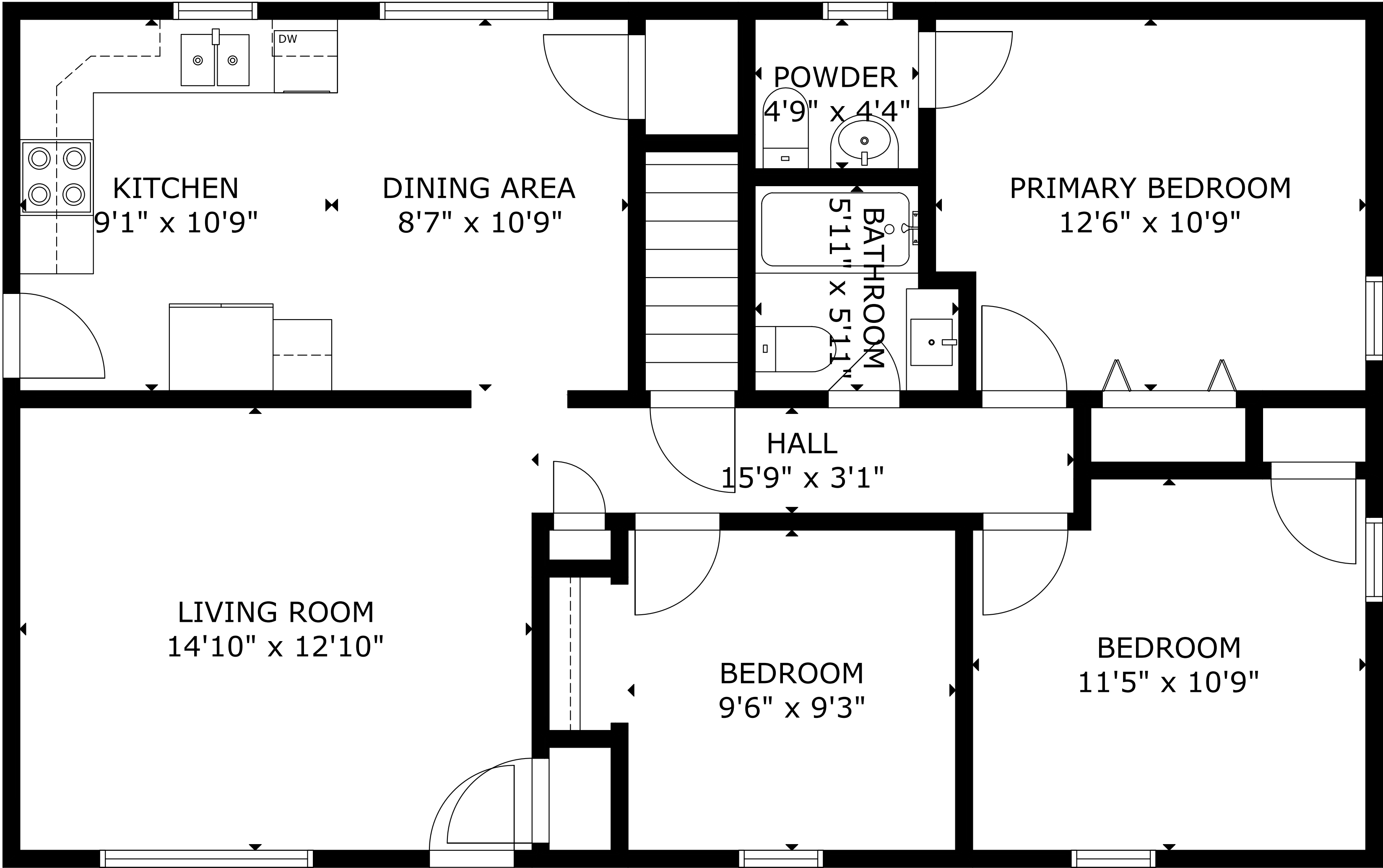
MAIN FLOOR
