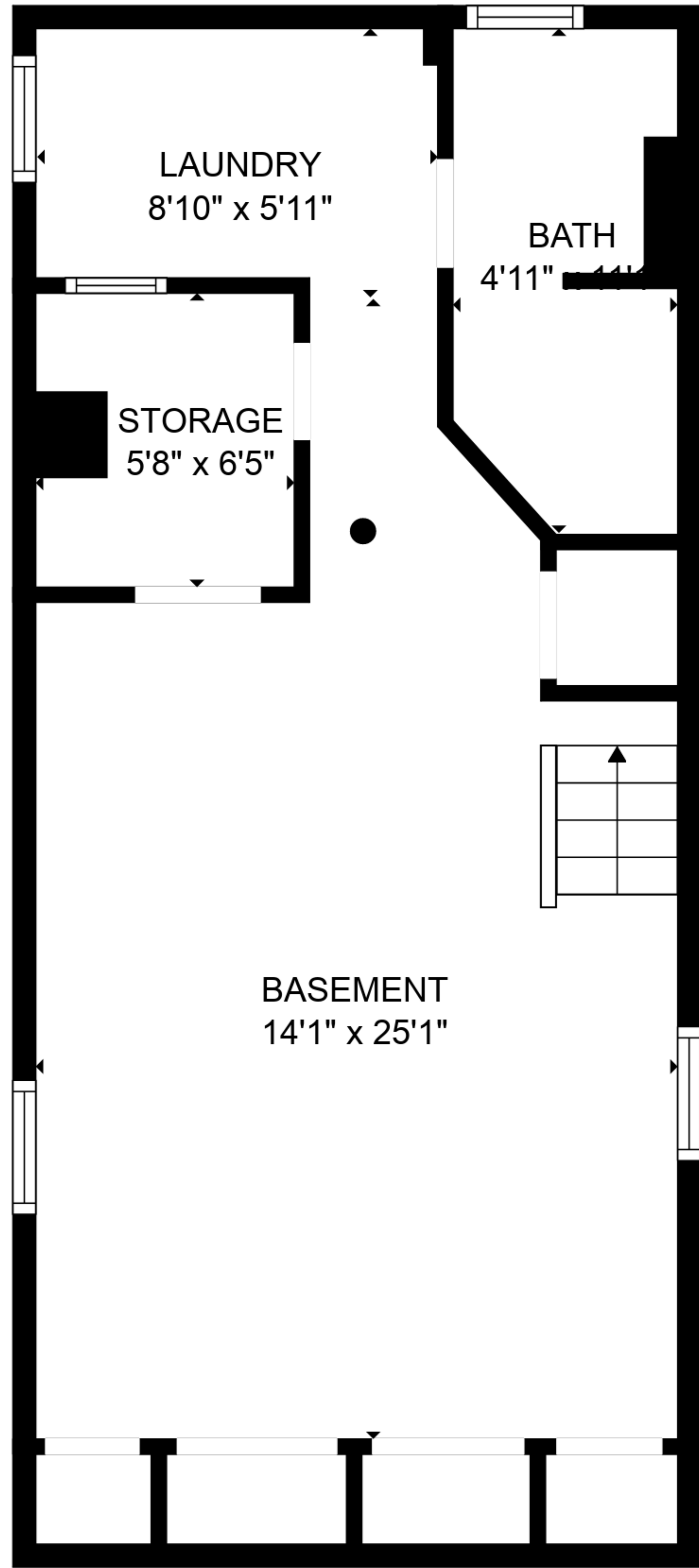
FLOOR 1
