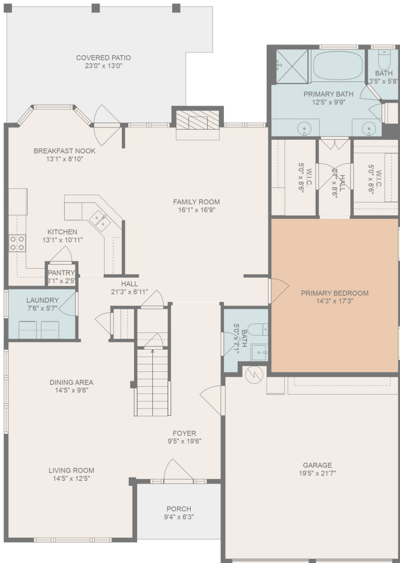
FLOOR 1
