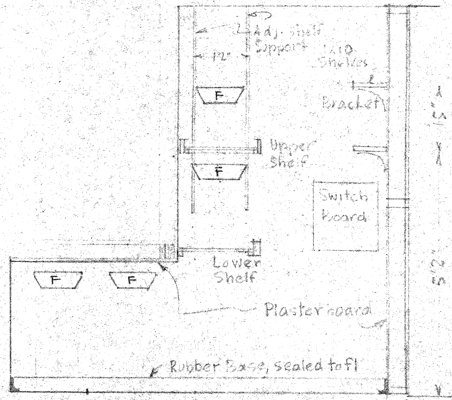
SECTION A-A 1/2" = 1 ft
