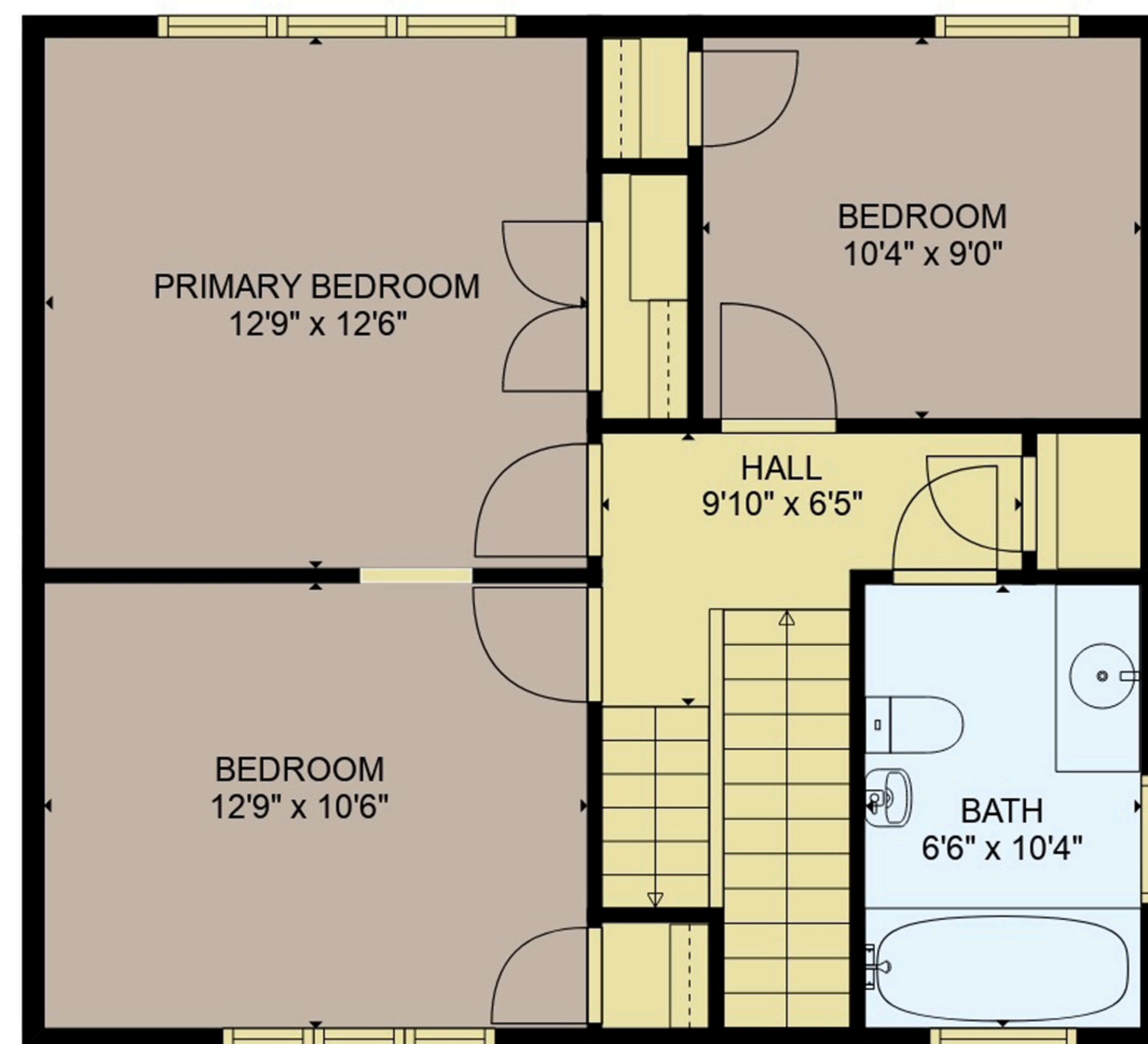
FLOOR 1
