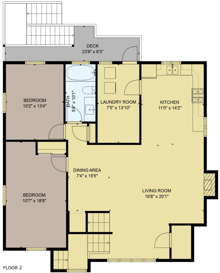
FLOOR 2
