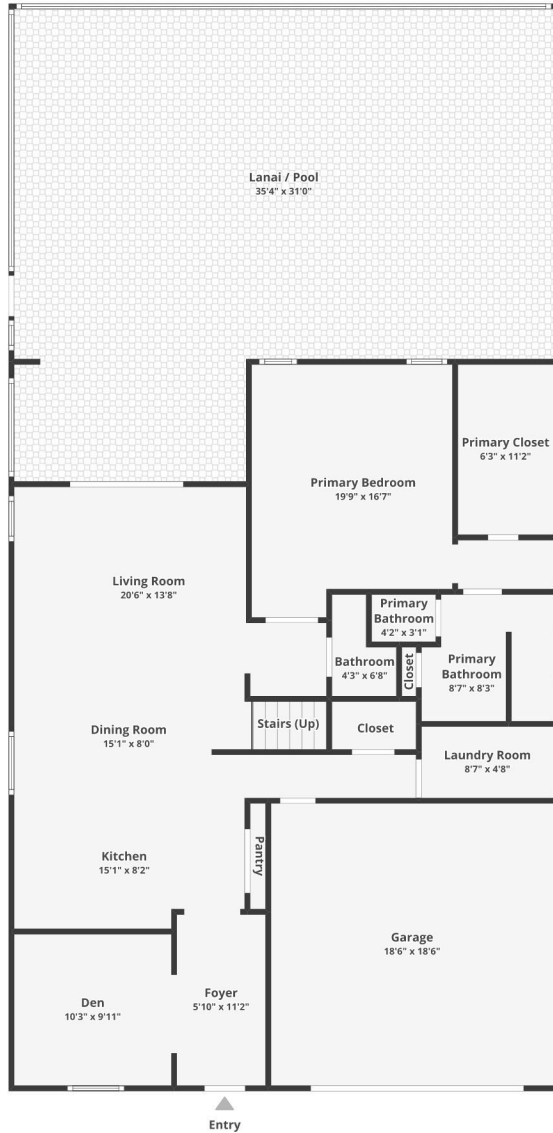
FLOOR 1
