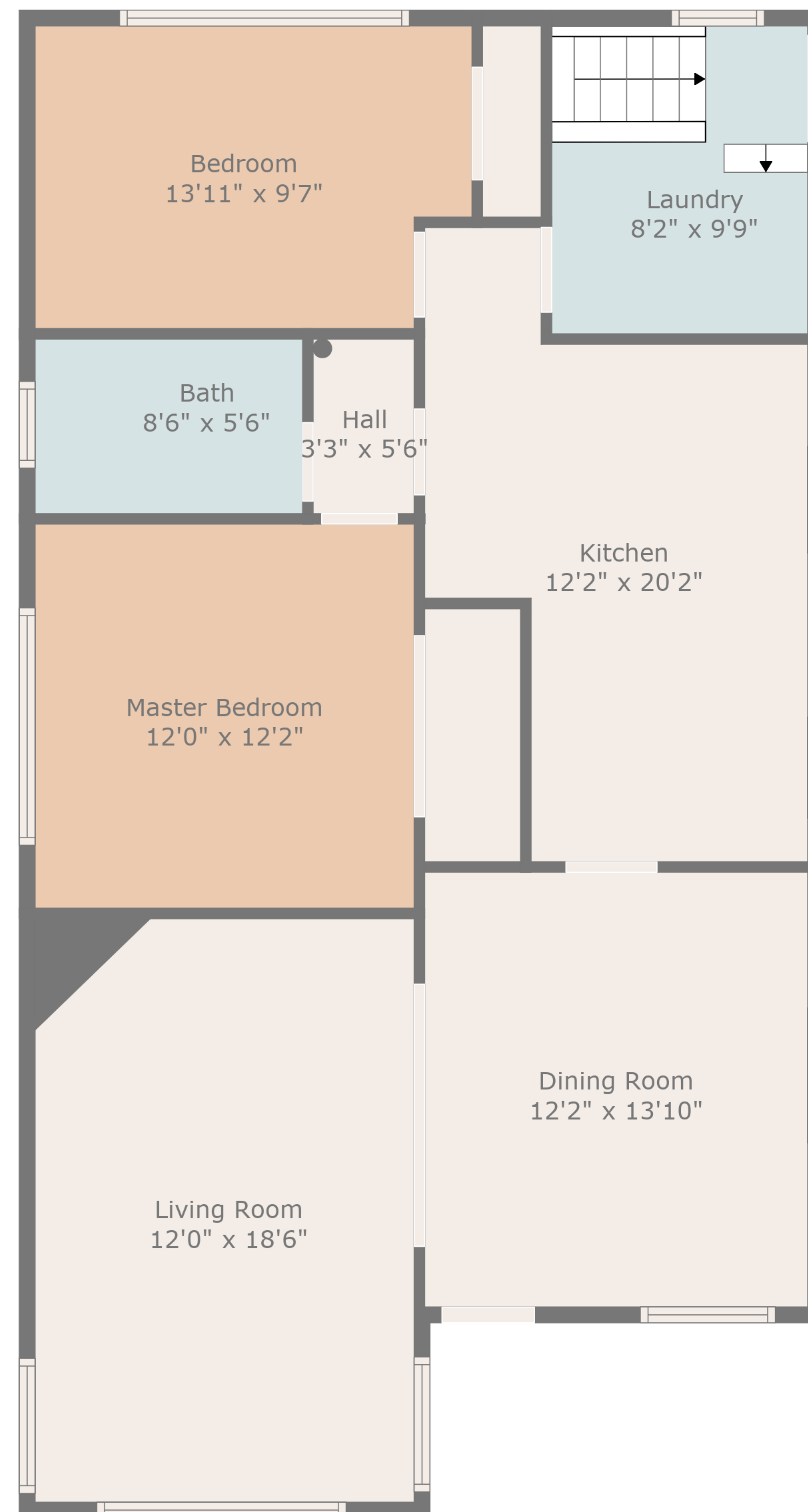
Floor 2
