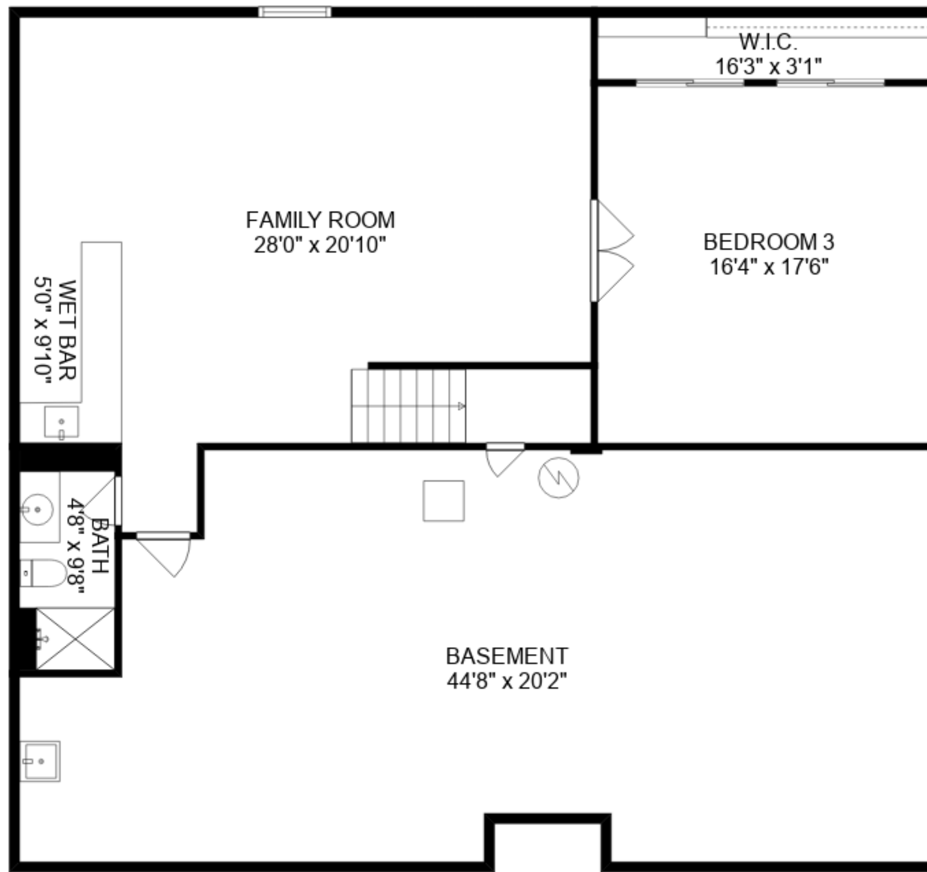
LOWER FLOOR
