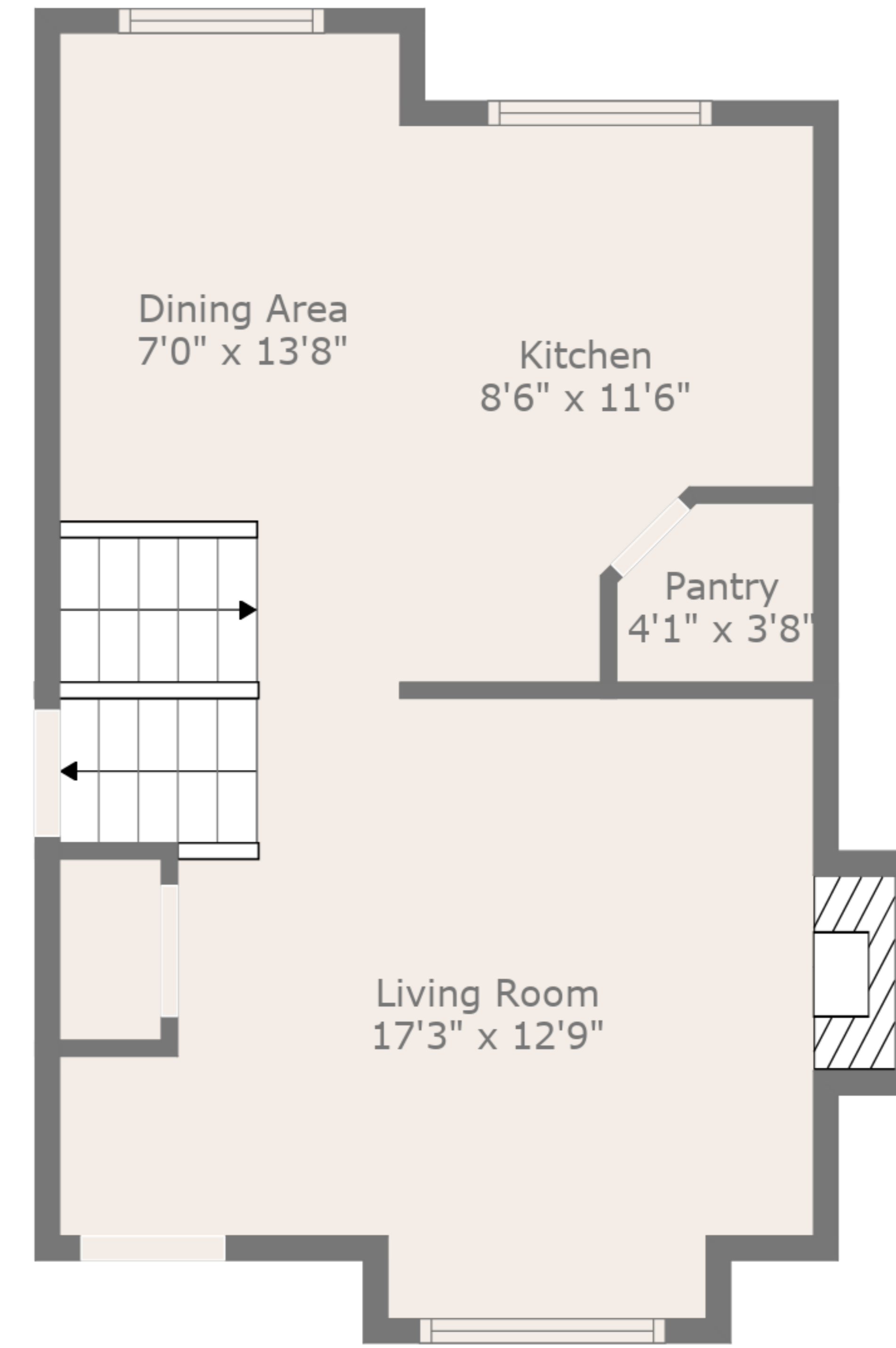
Floor 3
