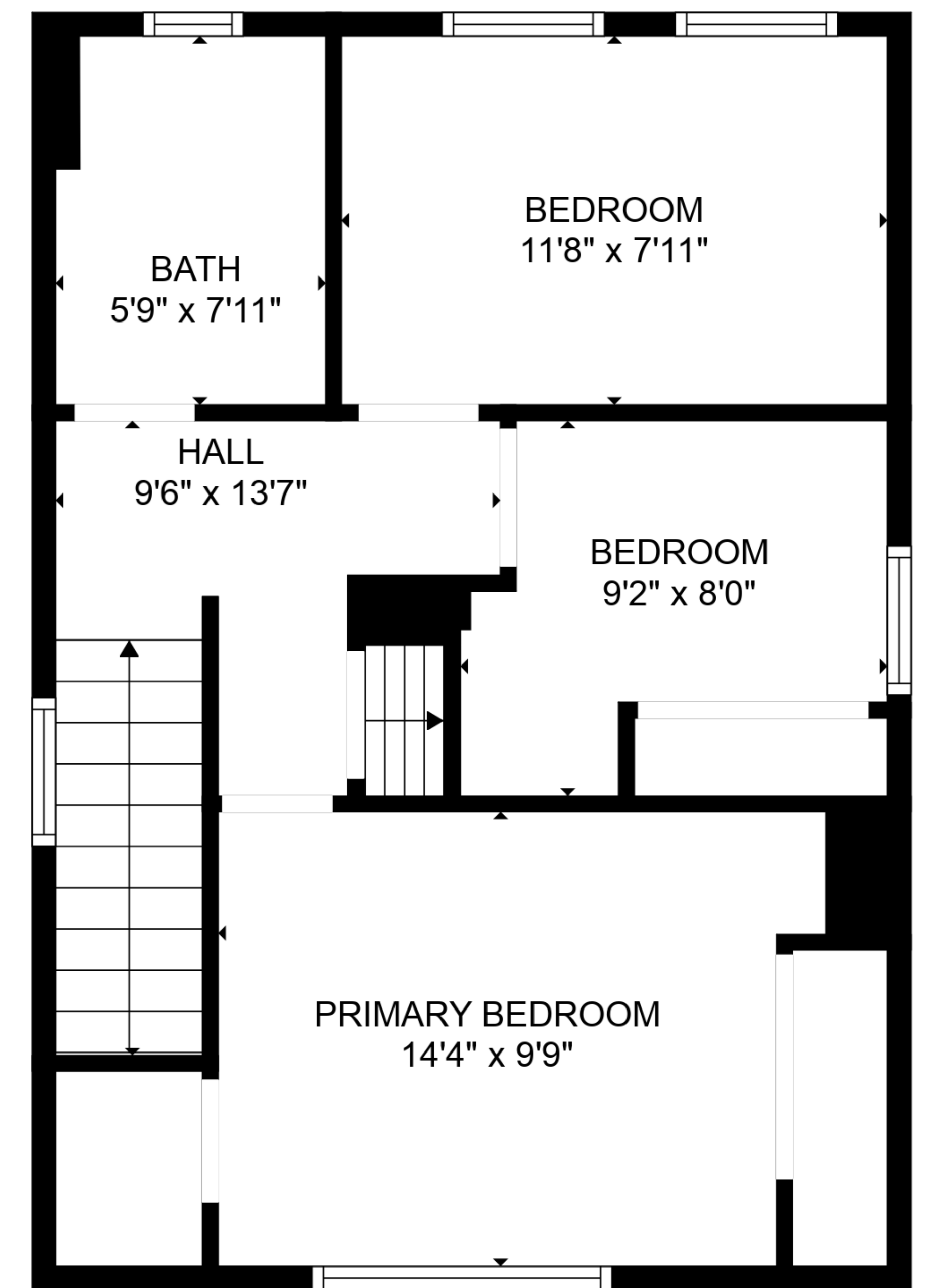
FLOOR 3
