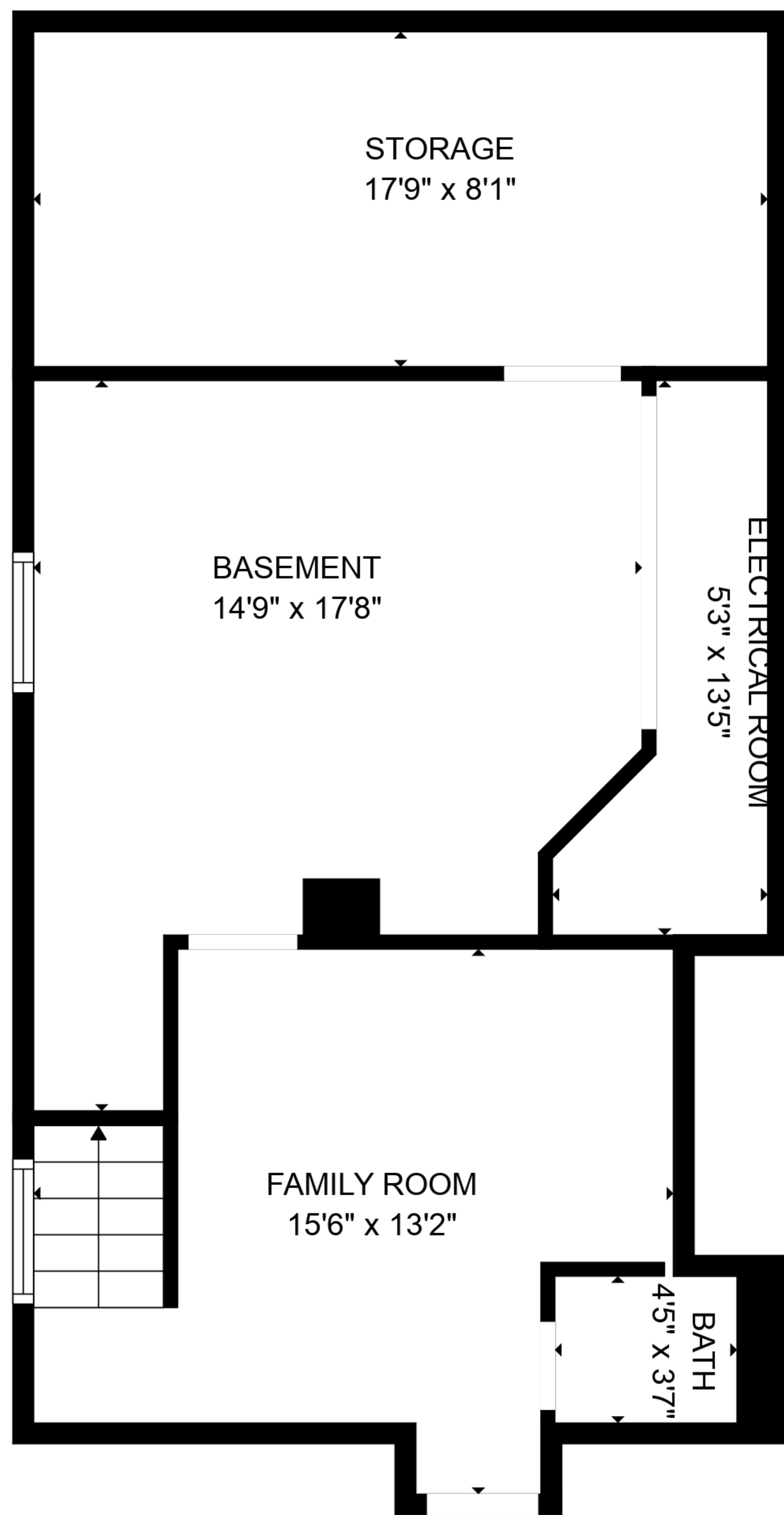
FLOOR 1
