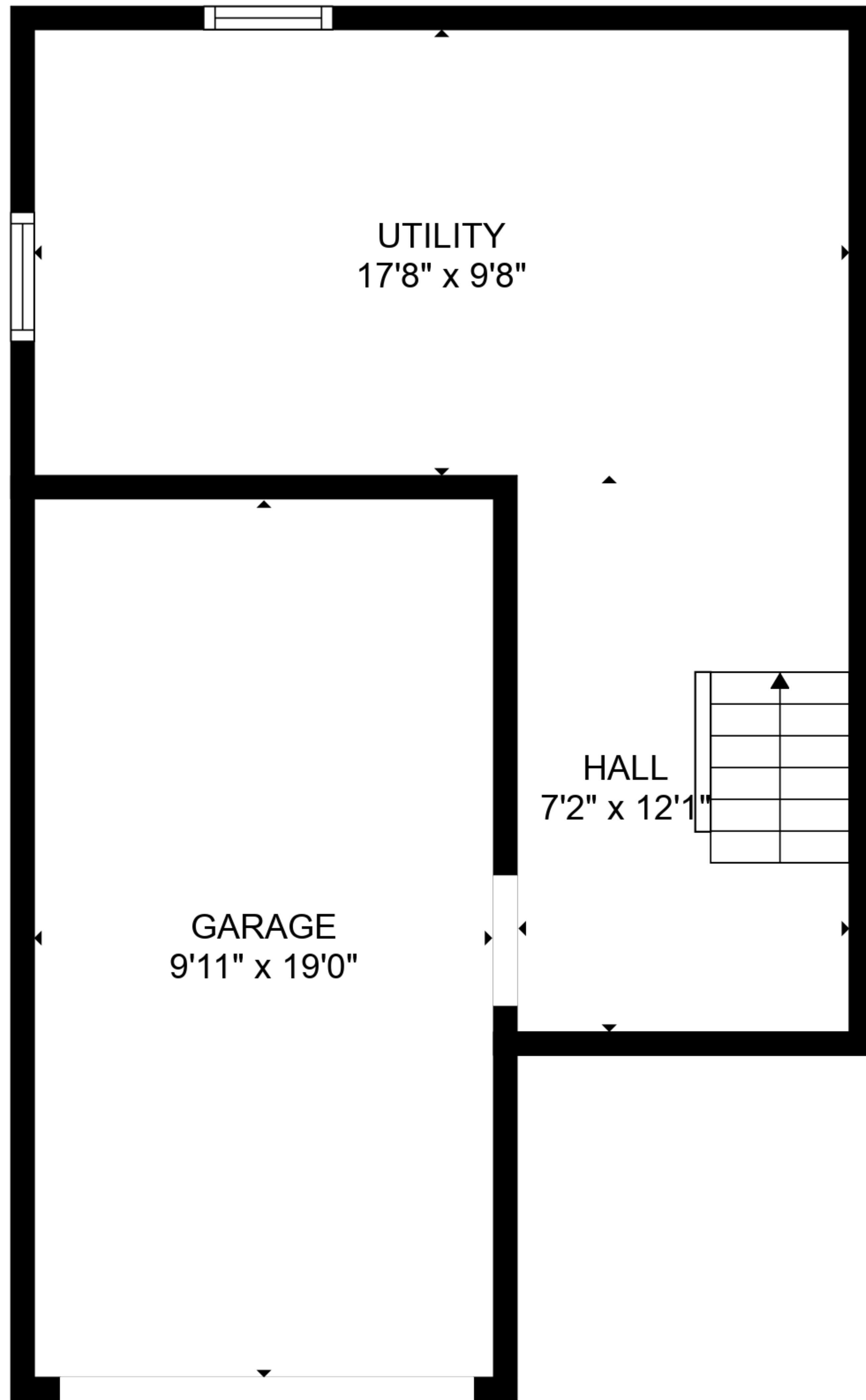
FLOOR 1
