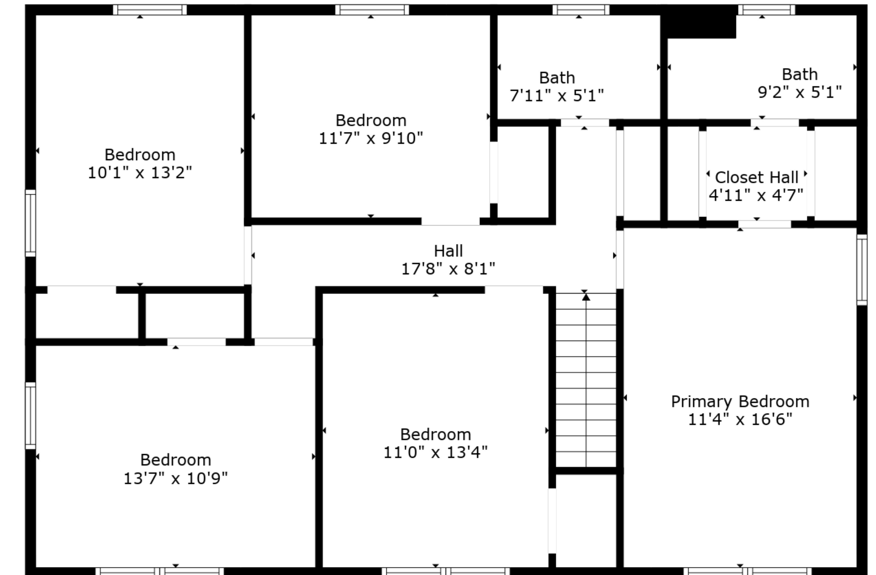
Floor 3
