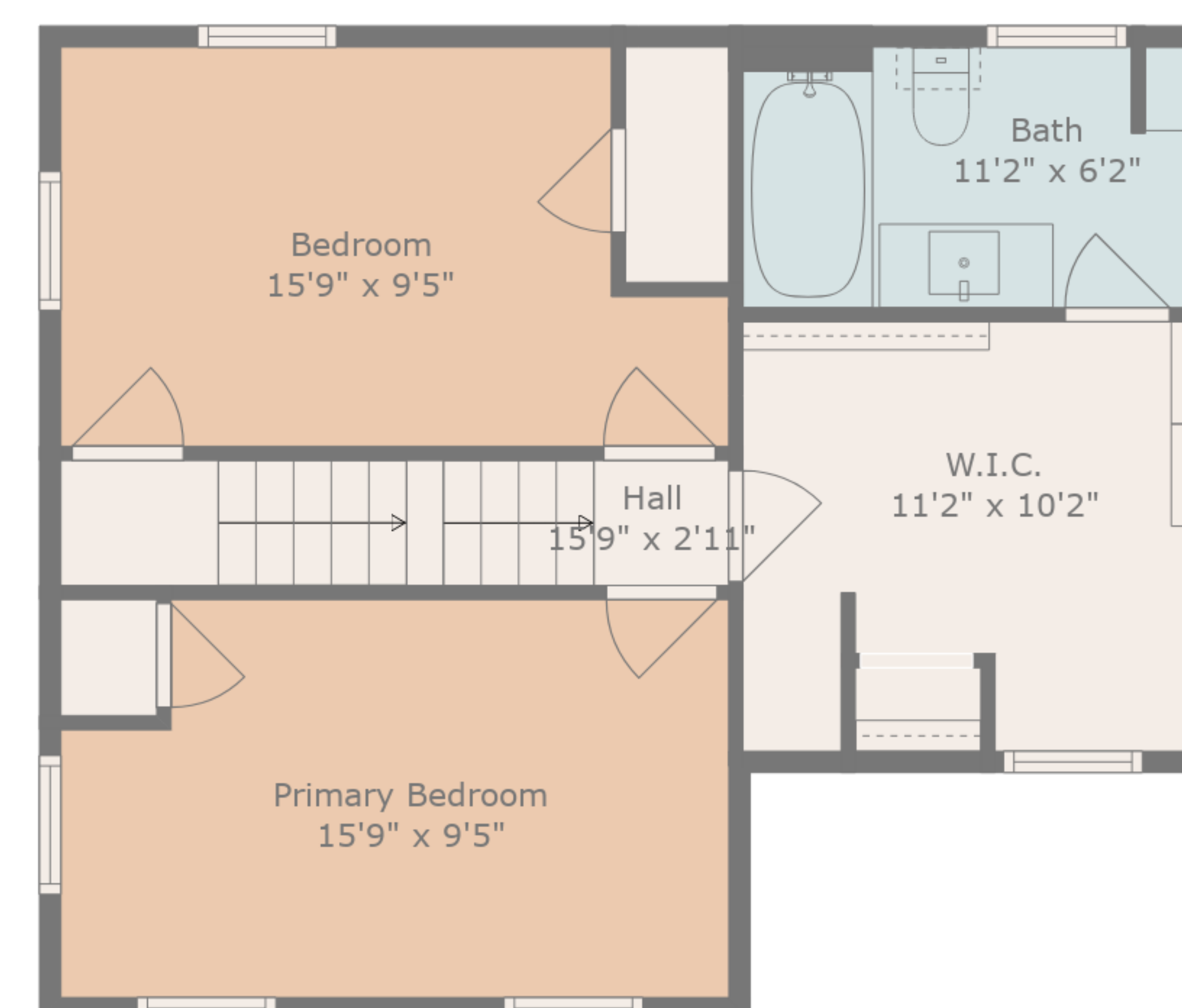
Floor 3
