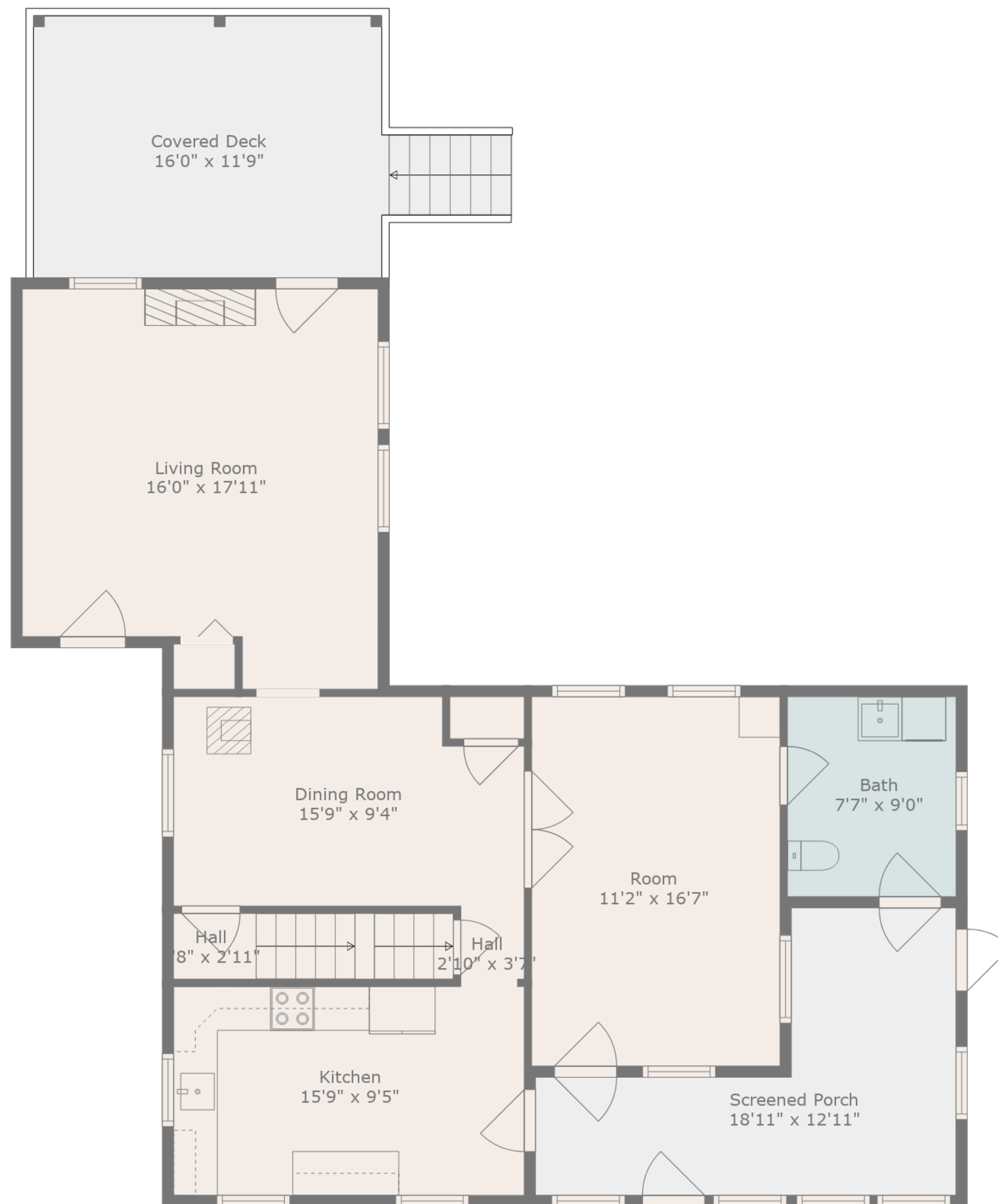
Floor 2
