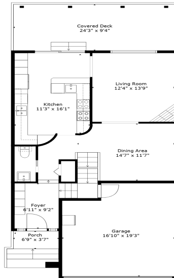
Floor 2
