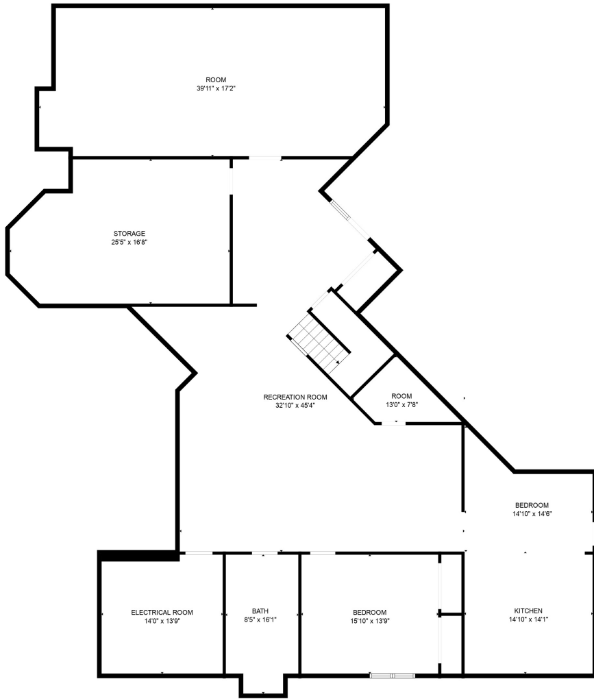
FLOOR 1
