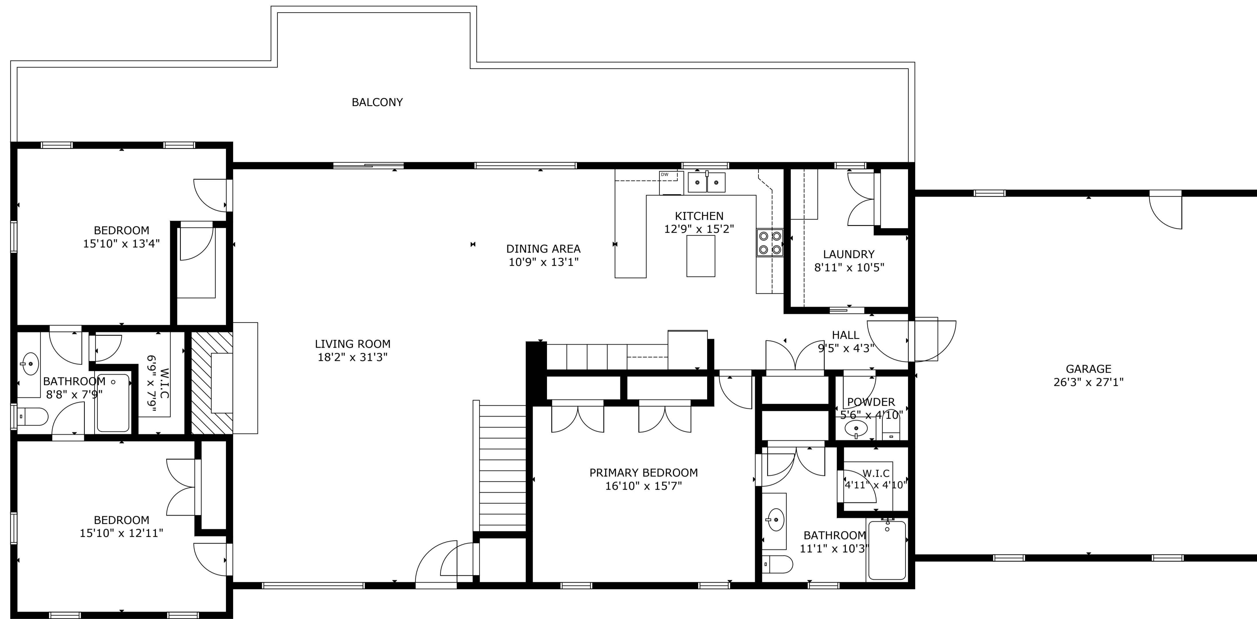
MAIN FLOOR
