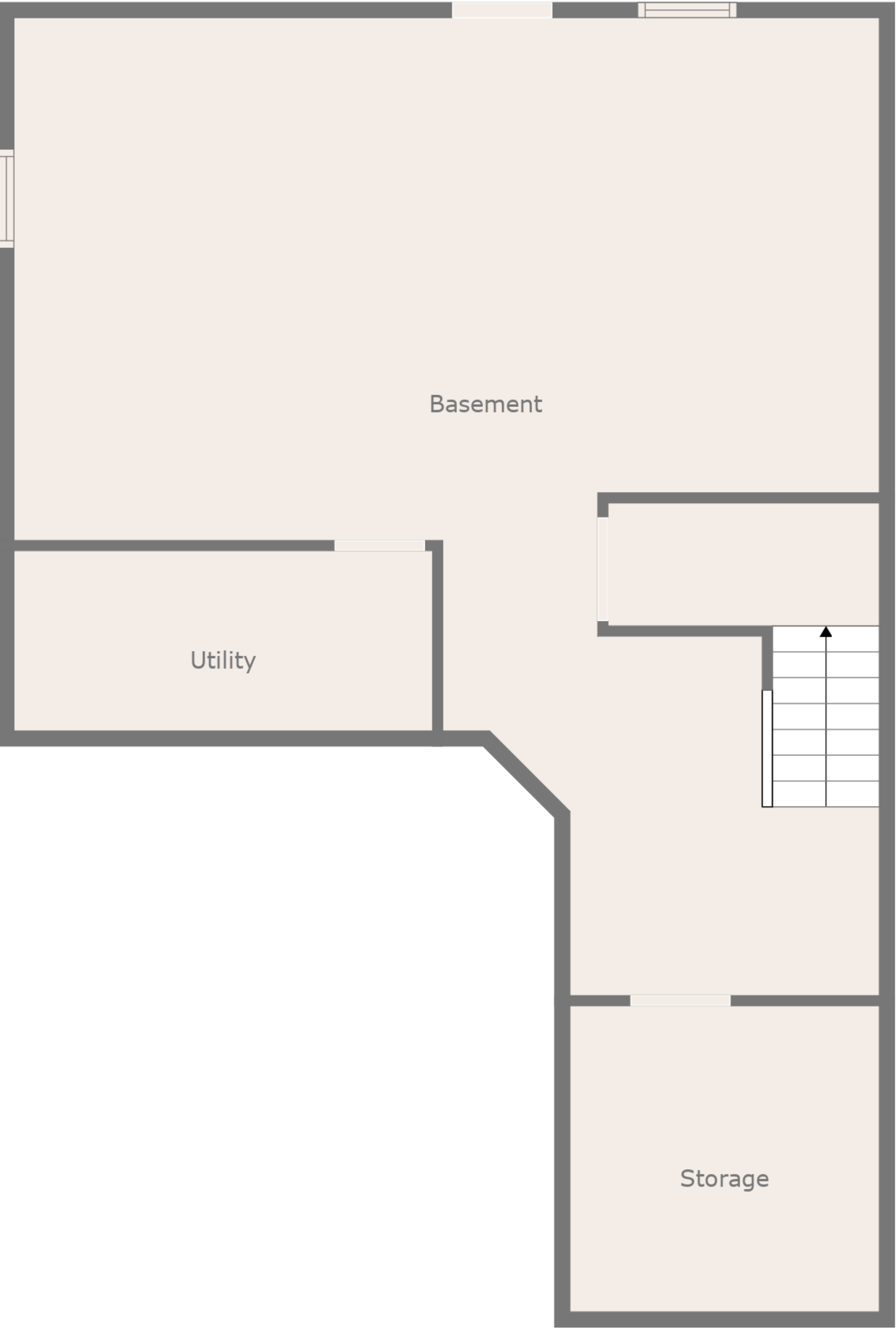
Floor 1
