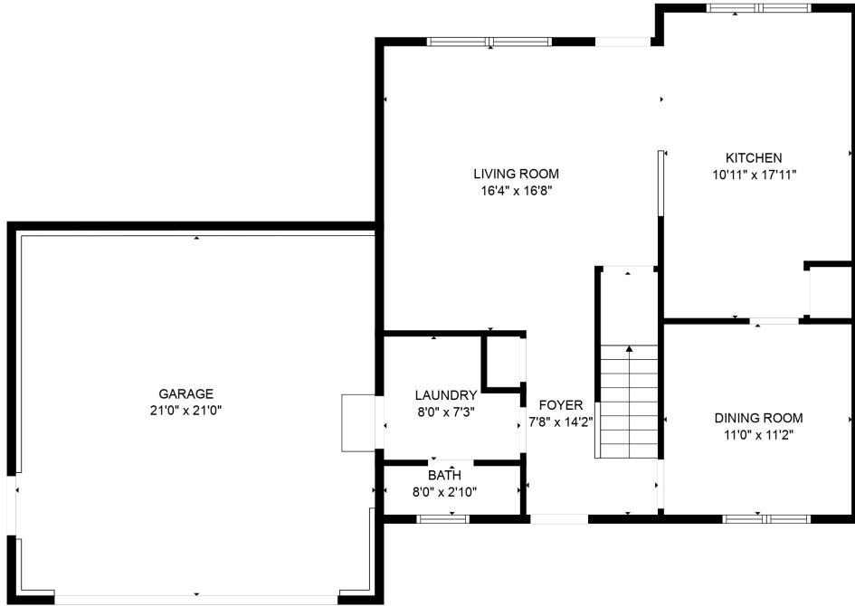
FLOOR 1
