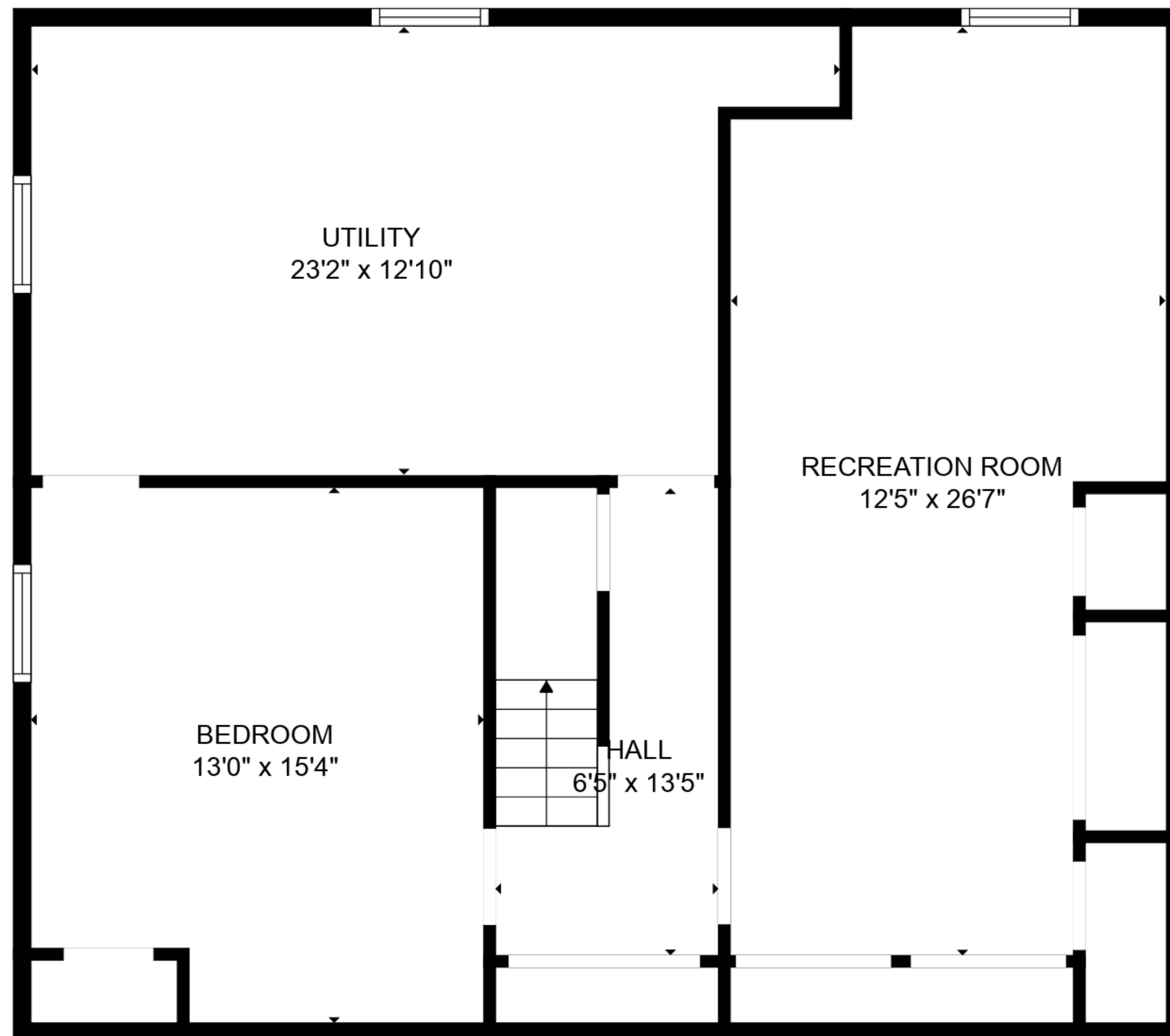
FLOOR 1
