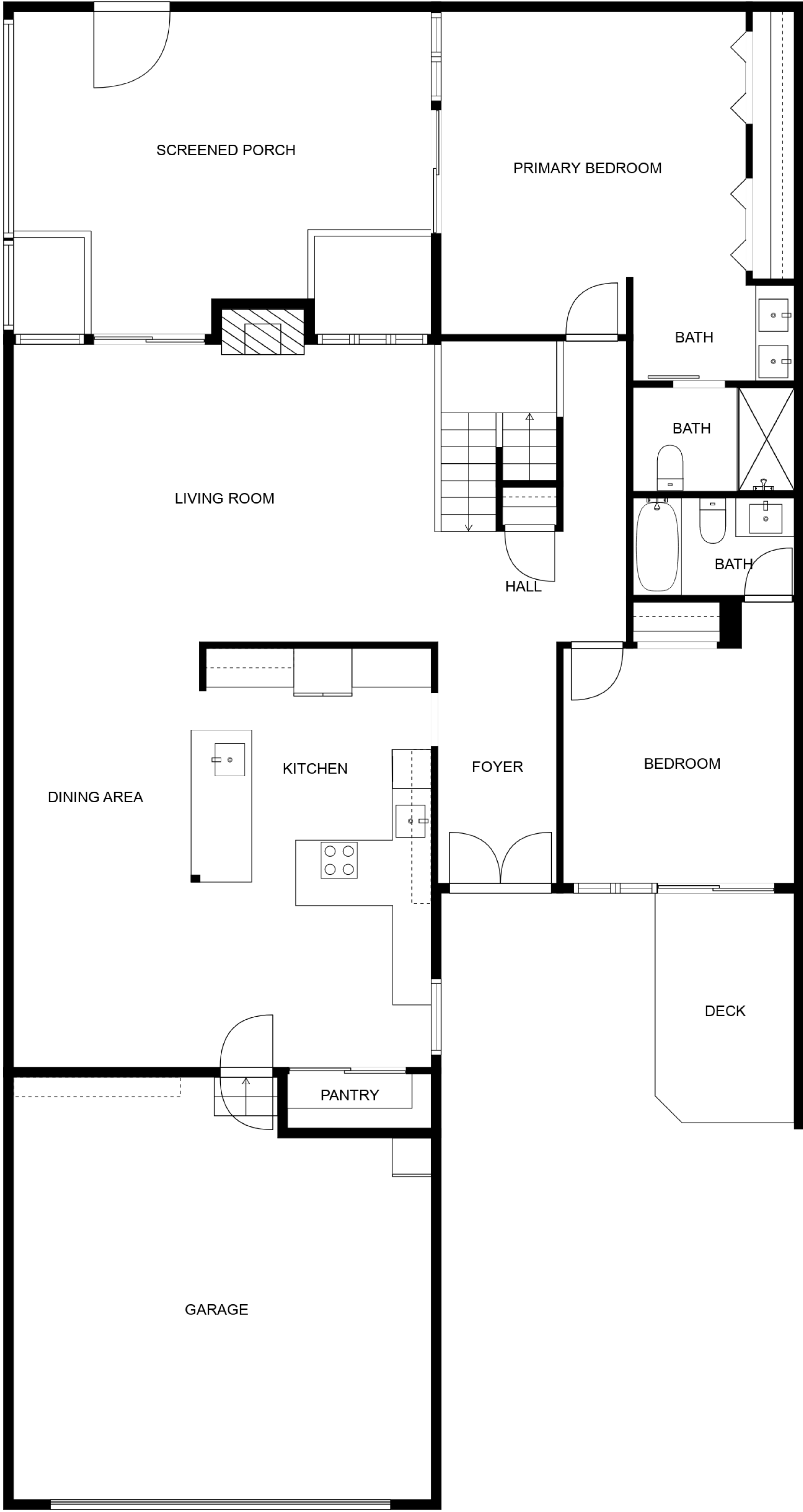
FLOOR 2
