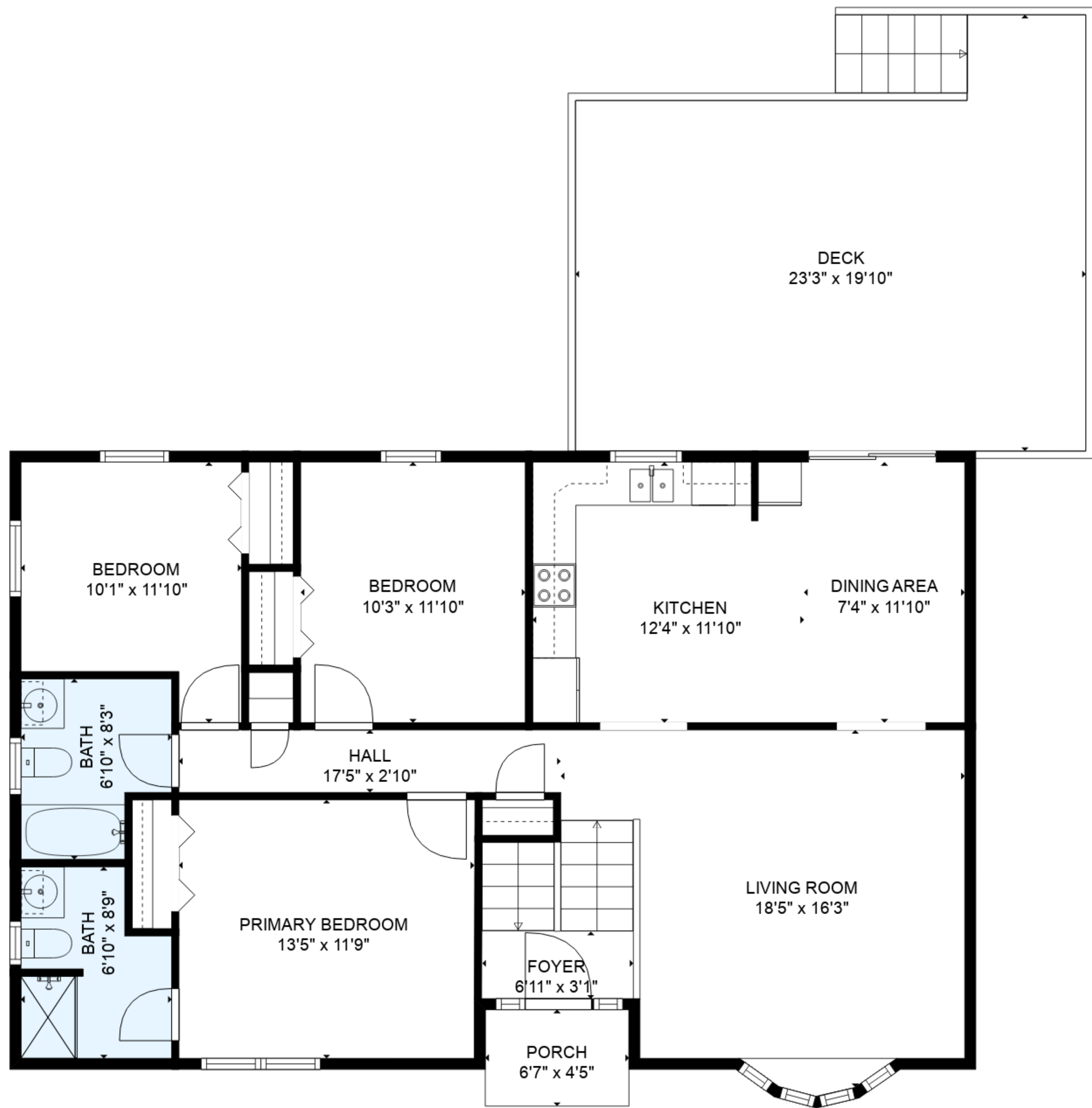
FLOOR 3
