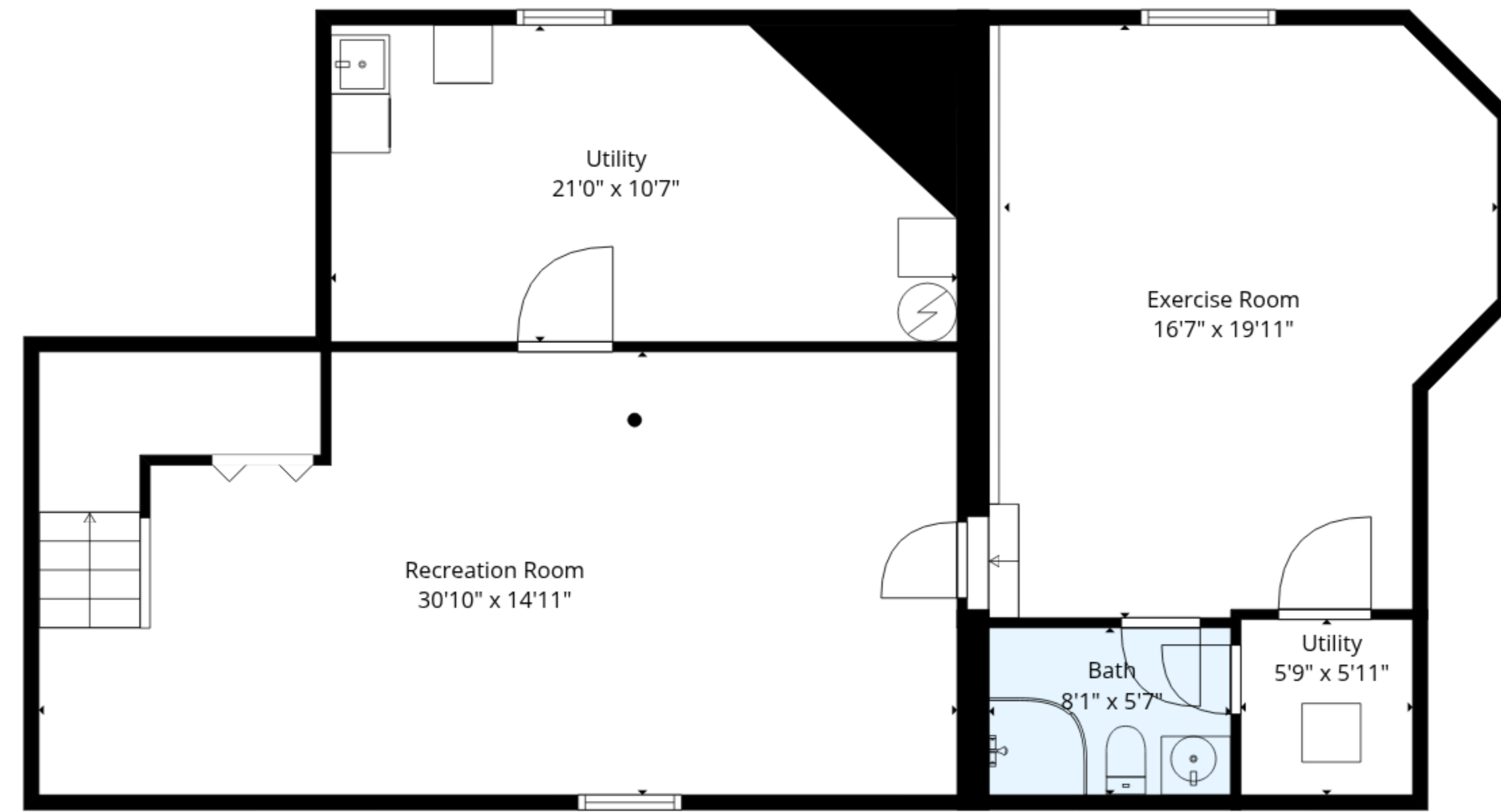
Basement
