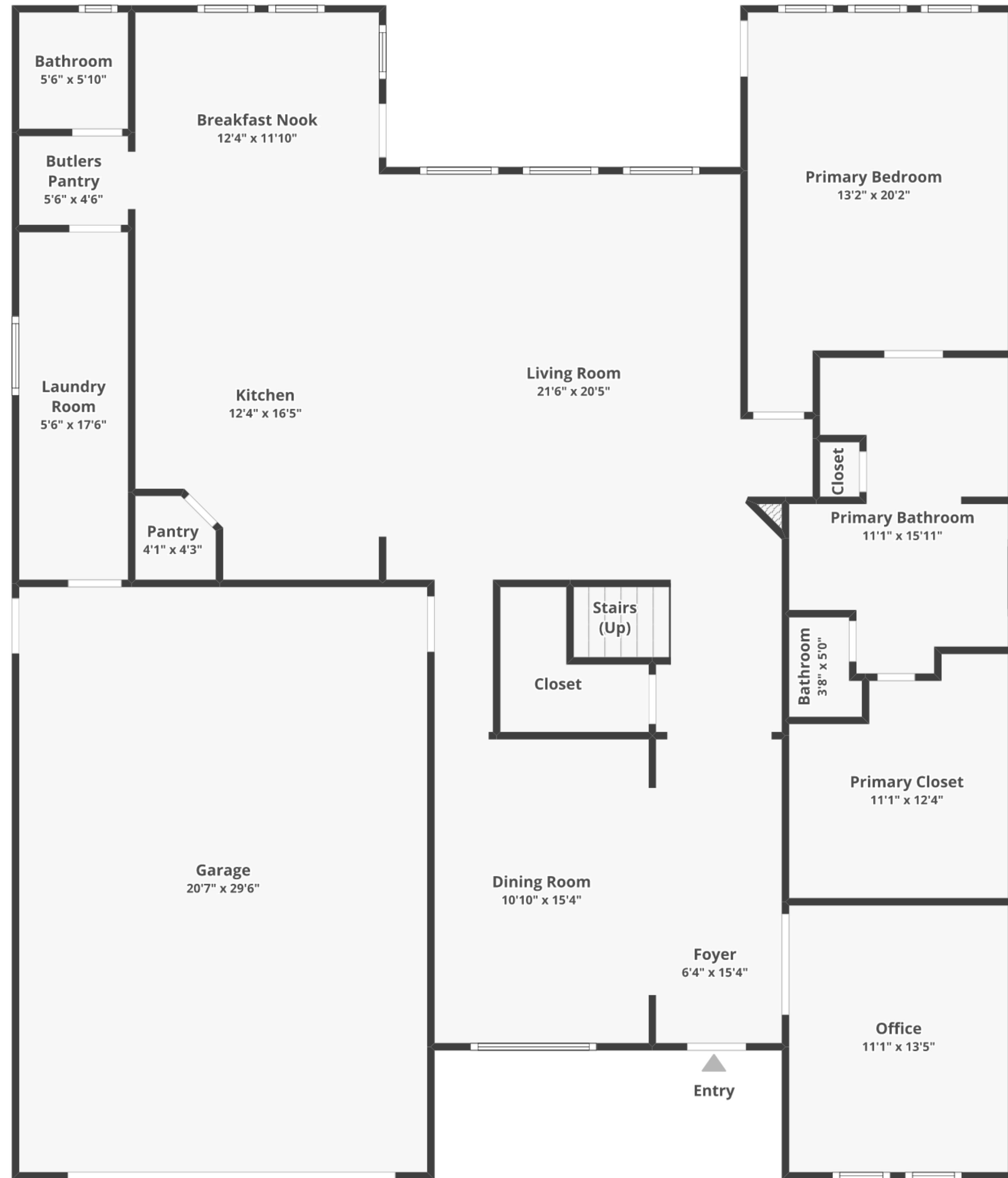
FLOOR 1
